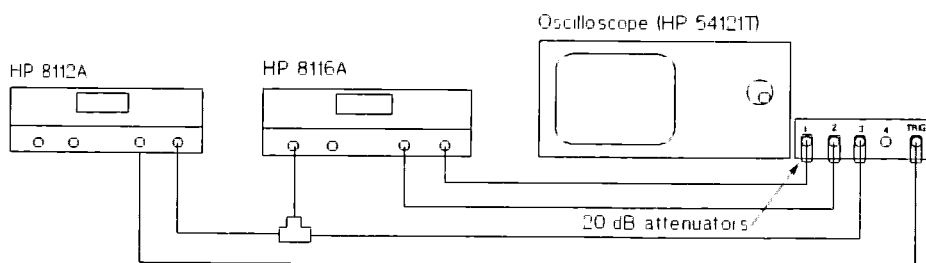
Figure 8-11. Trigger, Gate & External Width Performance Test
