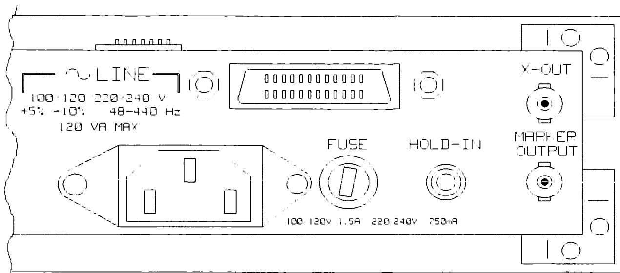
Figure 4-14. Rear panel
