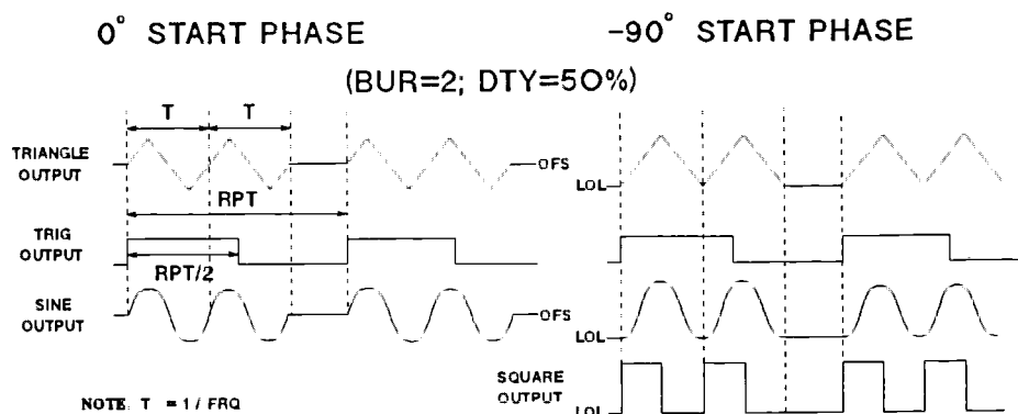
Figure 5-6. Typical outputs in Internal Burst mode
