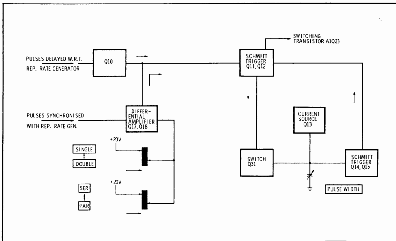
Figure 3-4. Delay Generator Block Diagram
