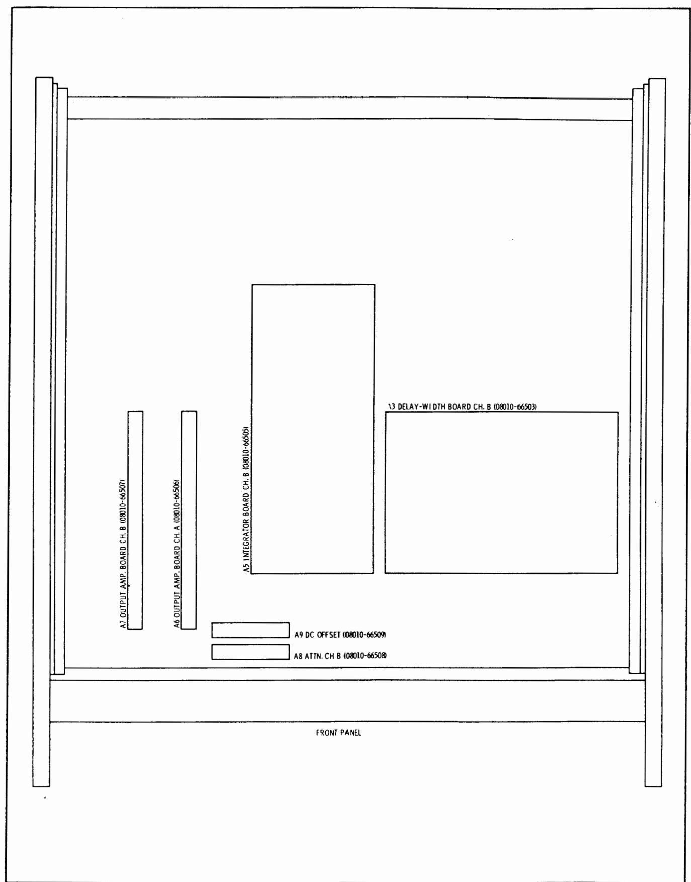
Figure 5-3. Bottom View
