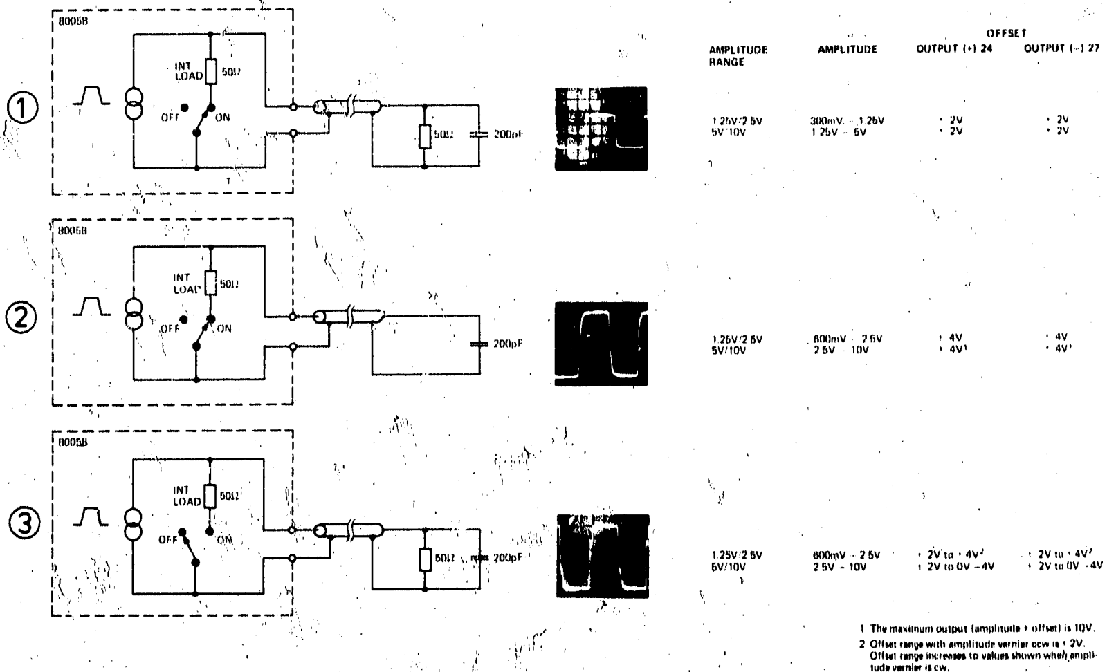
Figure 3-7. Output Configurations
