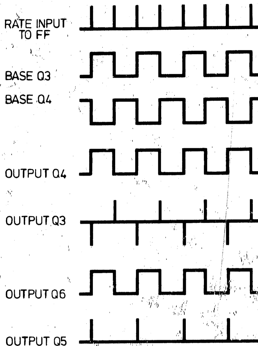
Figure 4-4. Square Wave Mode Timing Sequence
