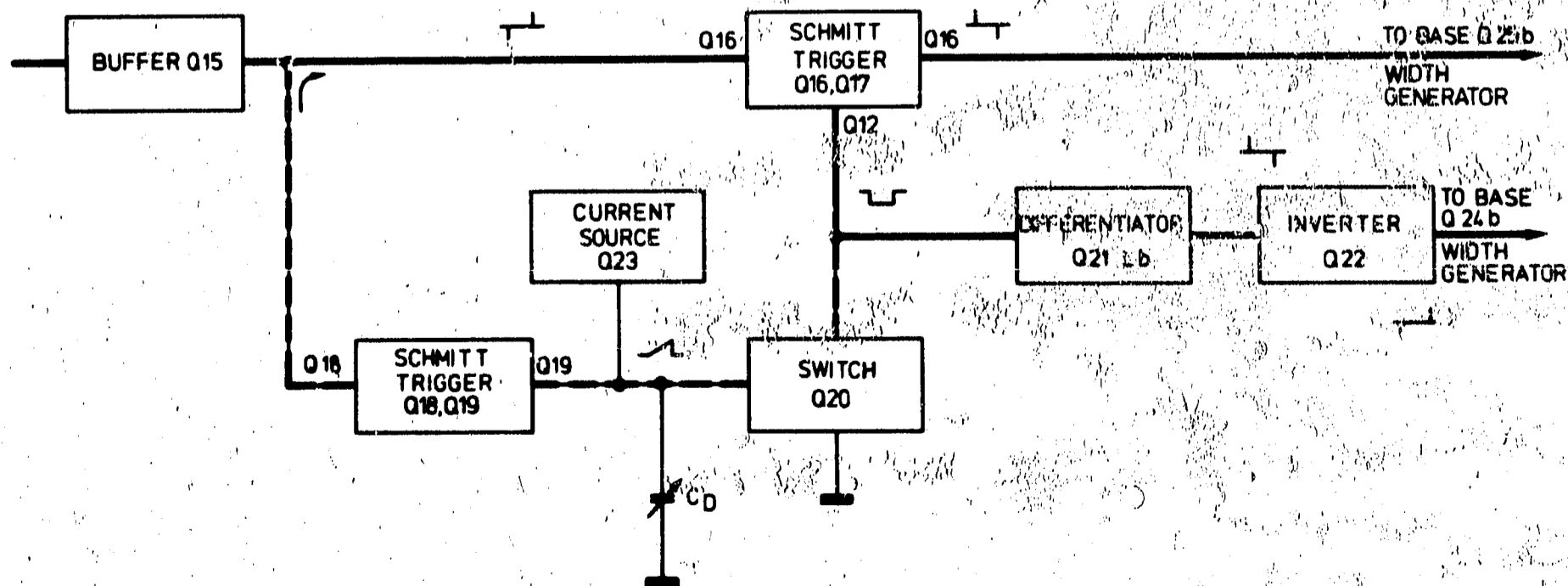
Figure 4-5. Delay Generator
