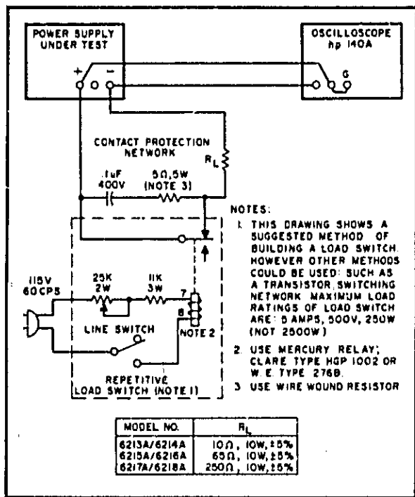
Figure 5-7. Transient Recovery Time, Test Setup
