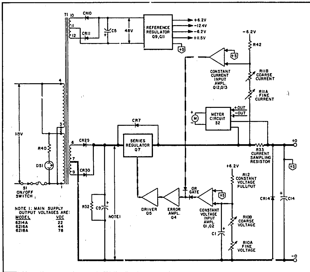
Figure 4-1. Block Diagram
