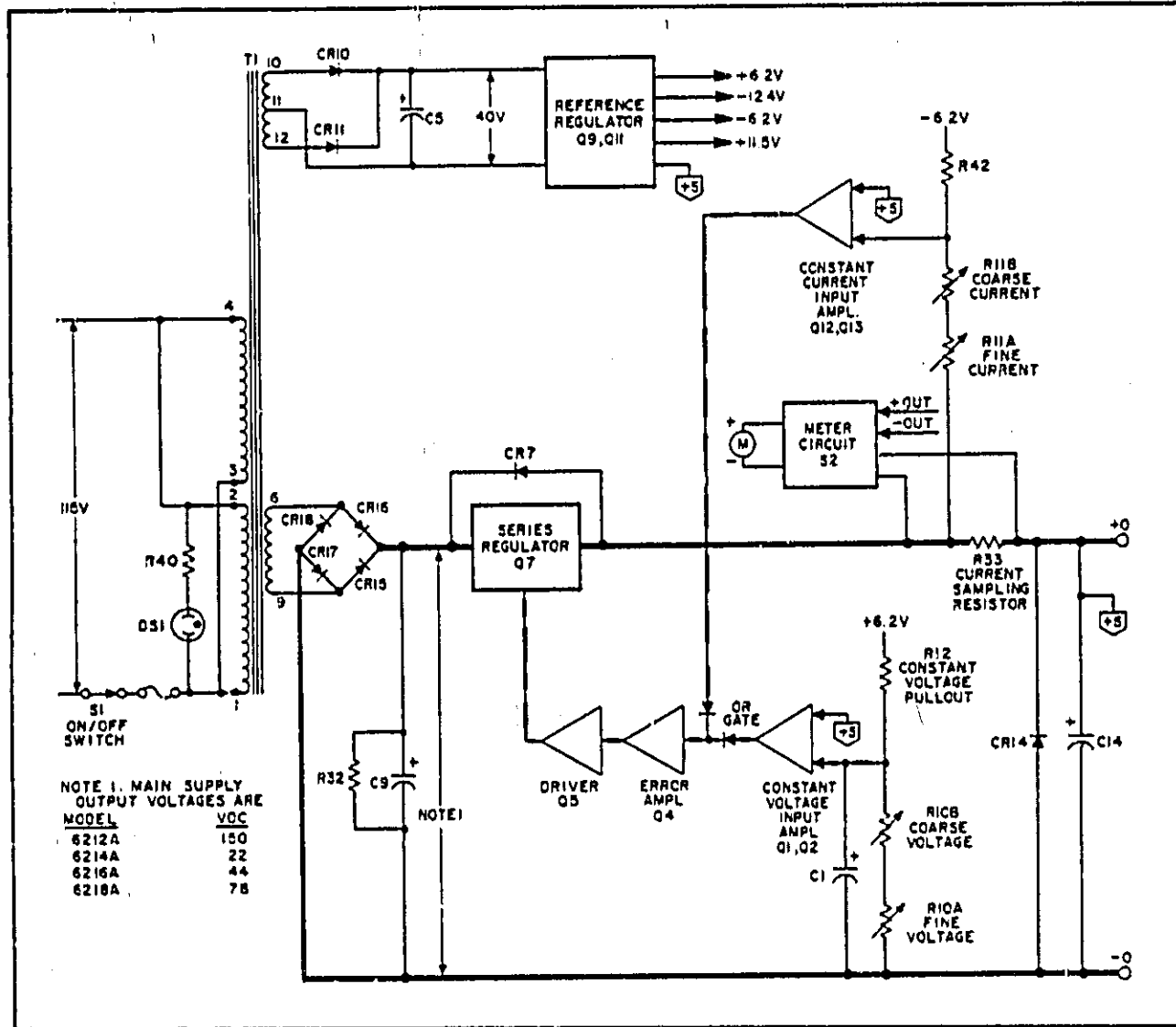
Figure 4-1. Block Diagram
