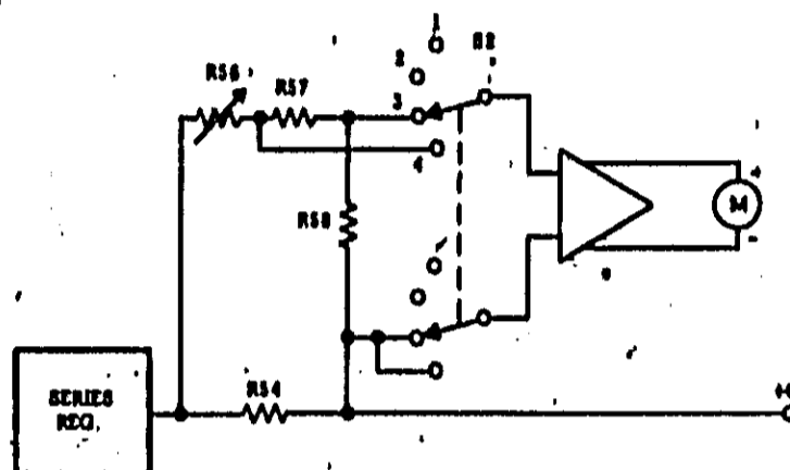
Figure 4-9. Ammeter Connections, Simplified Schematic
