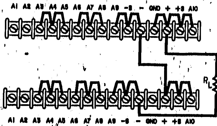
Figure 3-8. Normal Series
