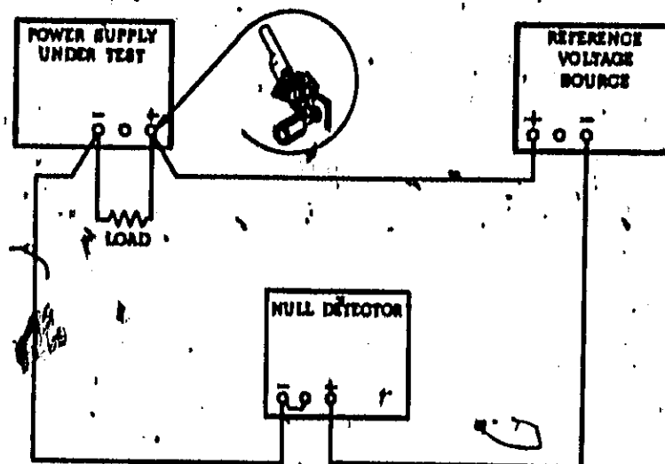
Figure 5-3. Differential Voltmeter Substitute, Test Setup
