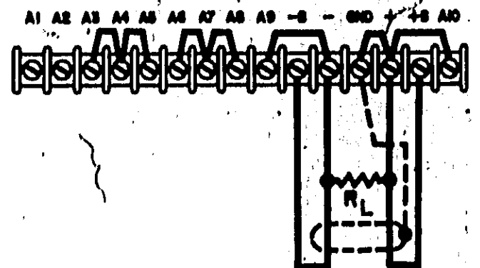
Figure 3-7. Remote Sensing
