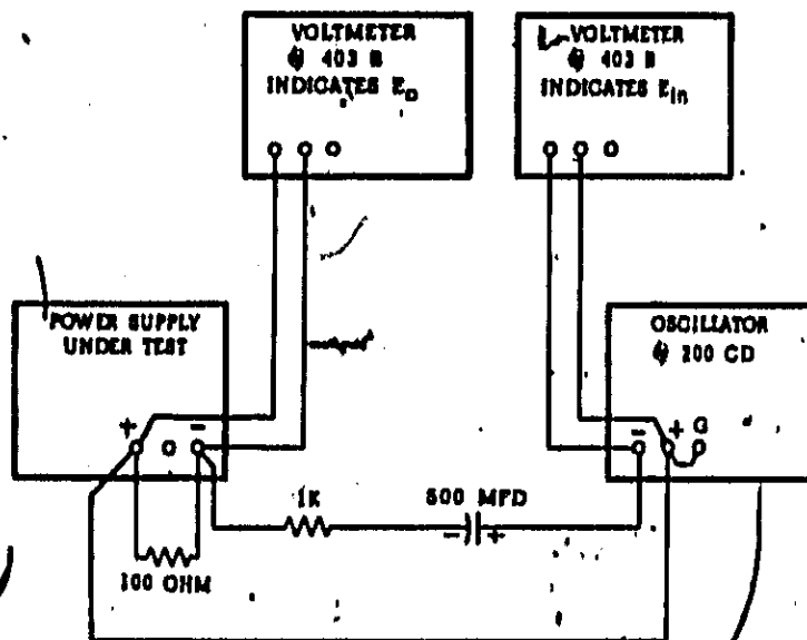
Figure 5-9. Output Impedance, Test Setup
