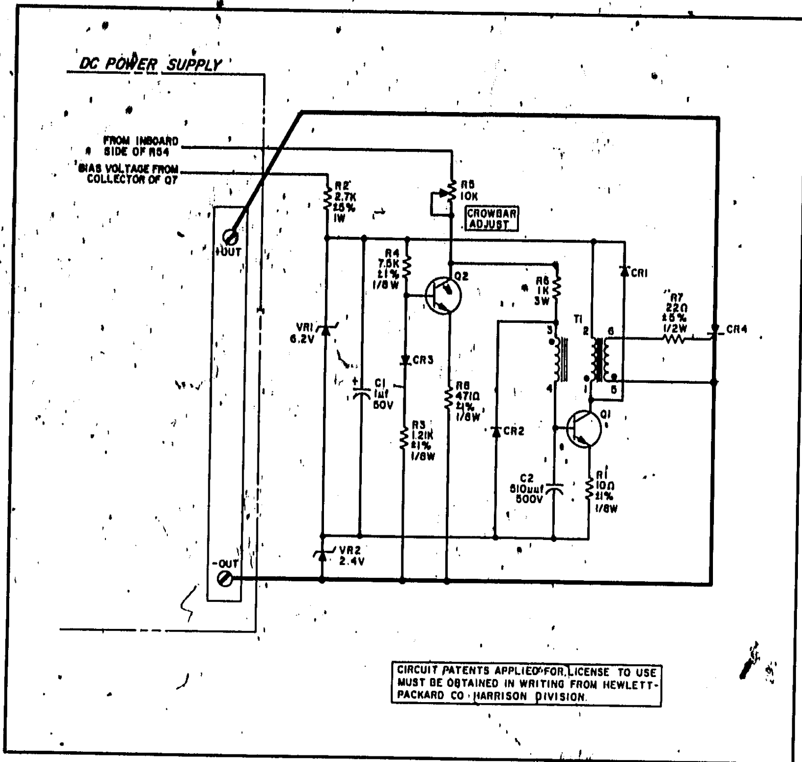
Figure A-1. Model 6201B Overvoltage Protection "Crowbar"
