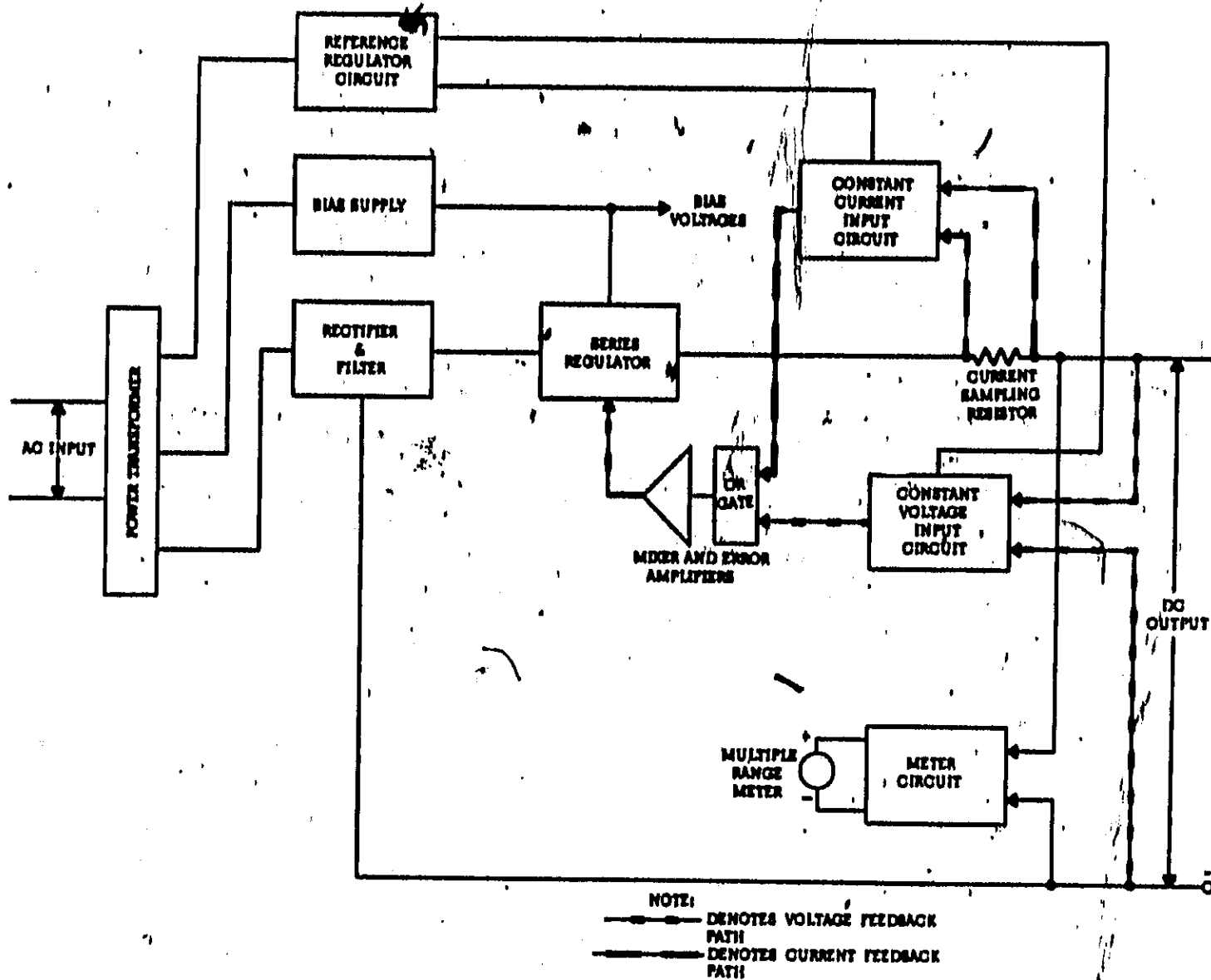
Figure 4-1. Overall Block Diagram
