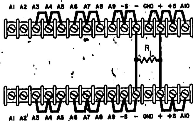
Figure 3-10. Normal Parallel
