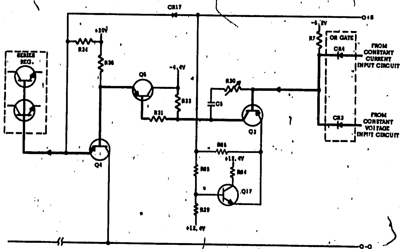
Figure 4-6. Mixer and Error Amplifiers, Simplified Schematic
