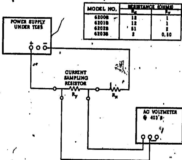
Figure 5-11. Ripple and Noise, Constant Current
