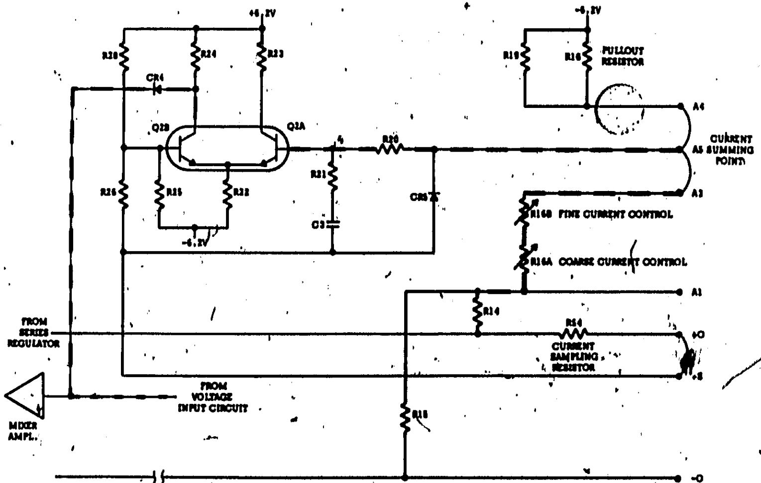
Figure 4-4. Constant Current Input Circuit, Simplified Schematic
