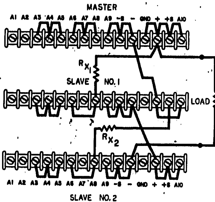
Figure 3-9. AUTO-Series, Two and Three Units
