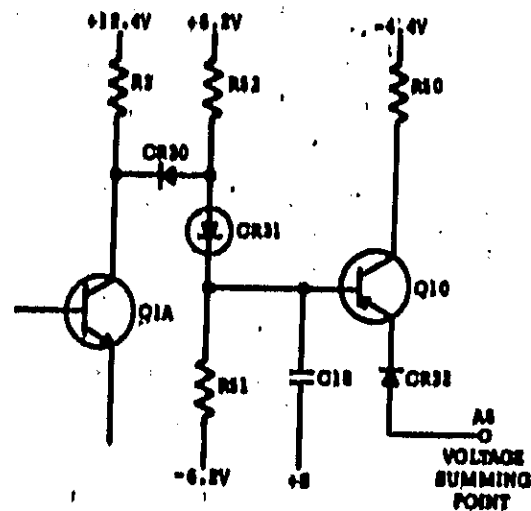
Figure 4-5. Voltage Clamp Circuit
