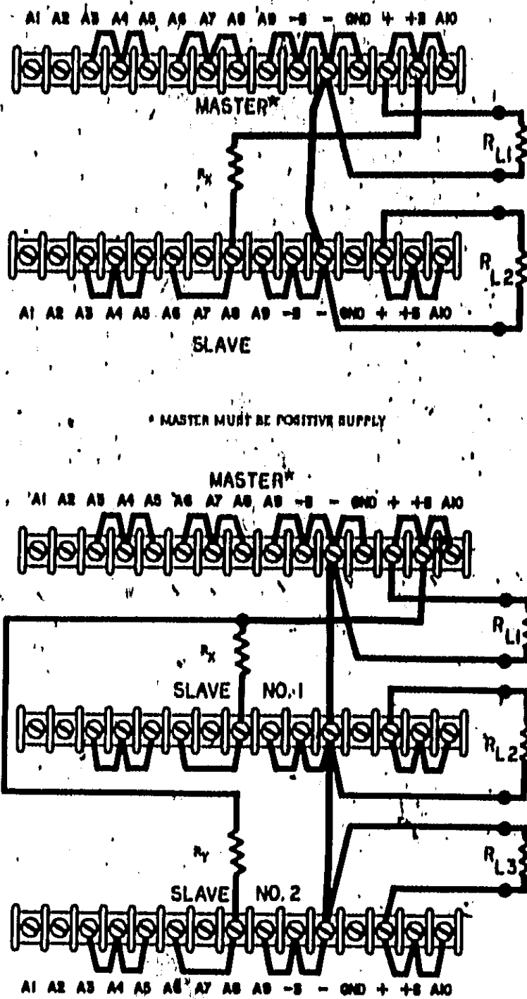
Figure 3-12. Auto-Tracking, Two and Three Units
