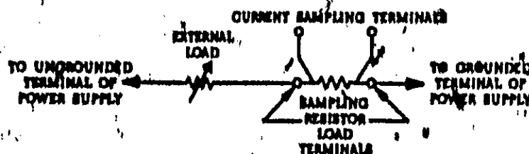
Figure 5-2. Output Current Measurement Technique
