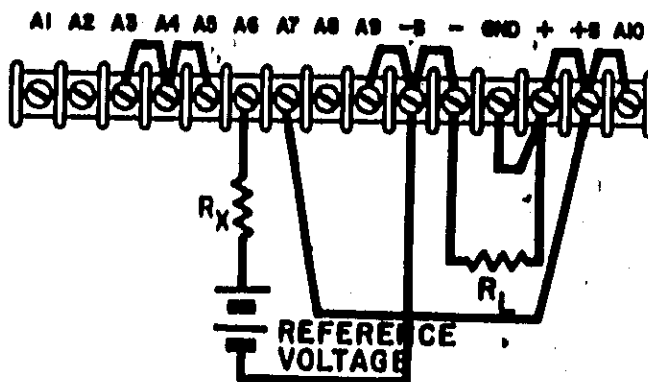
Figure 3-4. Remote Voltage Programming (Constant Voltage)
