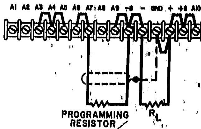
Figure 3-3. Remote Resistance Programming (Constant Voltage)
