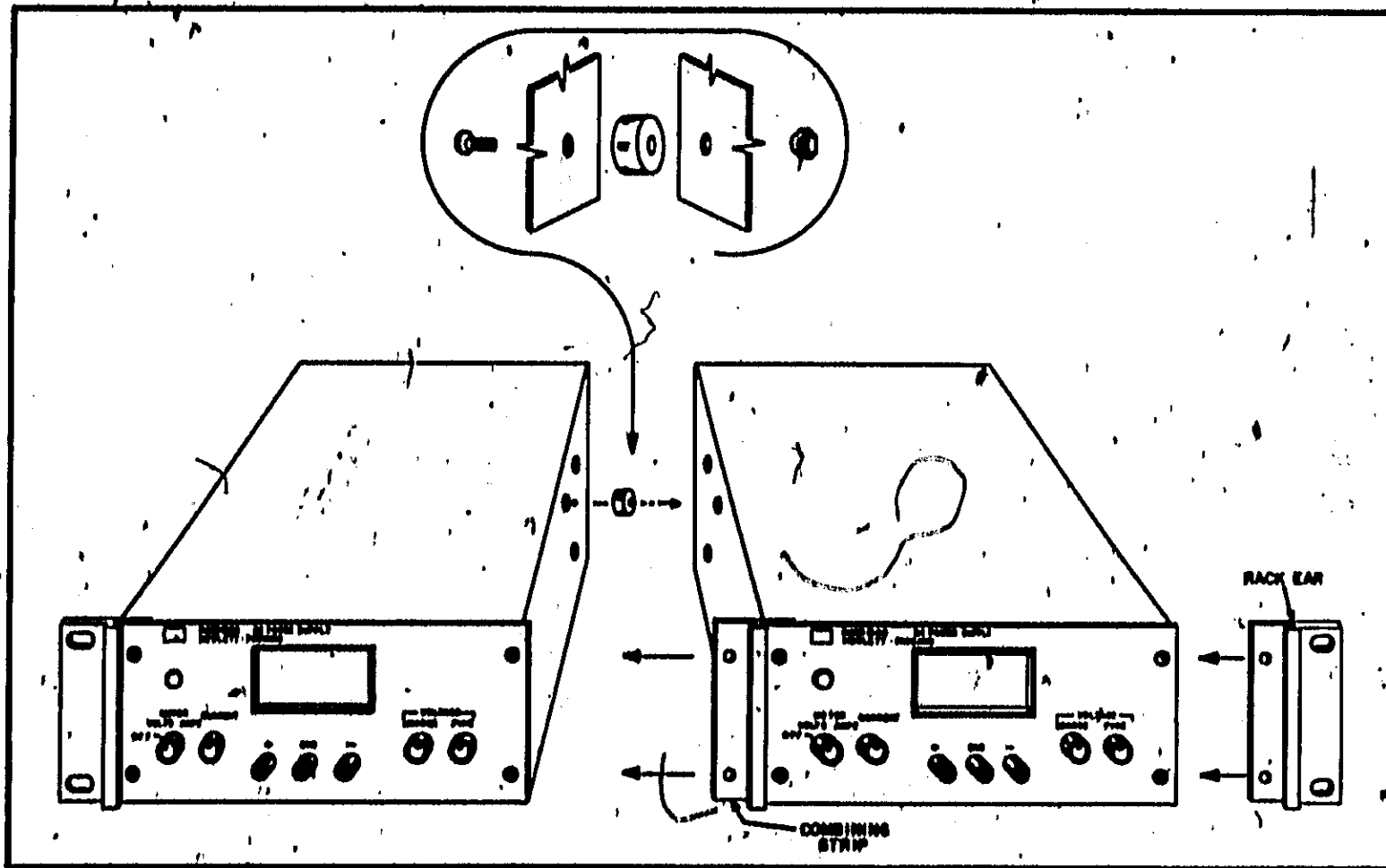
Figure 2-1: Rack Mounting, Two Units
