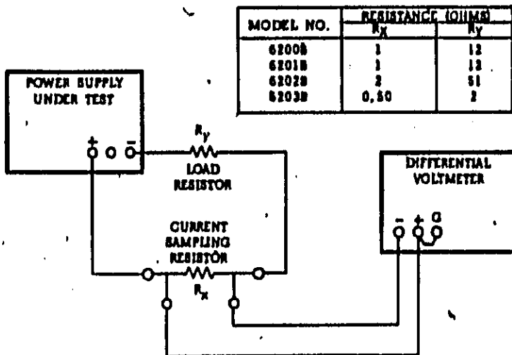
Figure 5-4. Output Current, Test Setup
