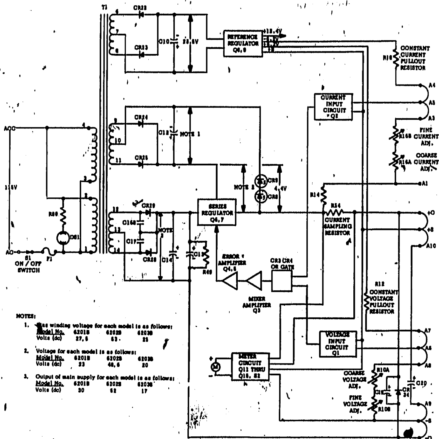
Figure 4-2. Simplified Schematic
