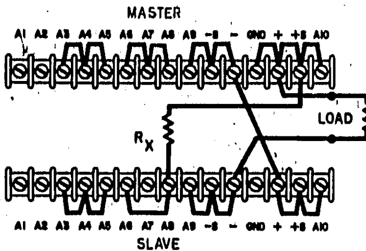
Figure 3-8. Normal Series
