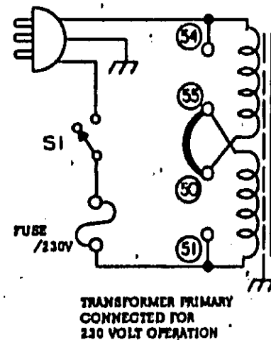
Figure 2-3. Primary Connections
