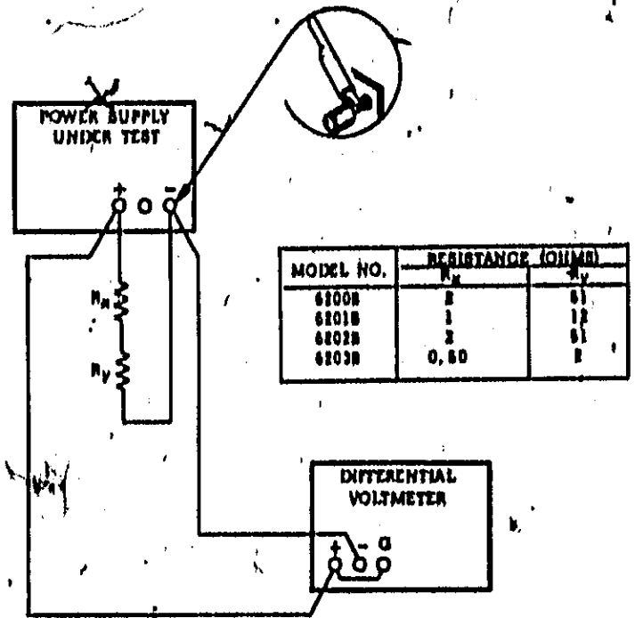
Figure 5-5. Load Regulation, Constant Voltage
