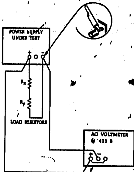
Figure 5-6. Ripple and Noise, Constant Voltage
