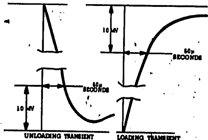
Figure 5-8. Transient Response, Waveforms
