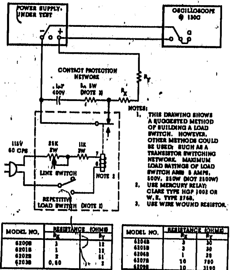
Figure 5-7. Transient Response, Test Setup
