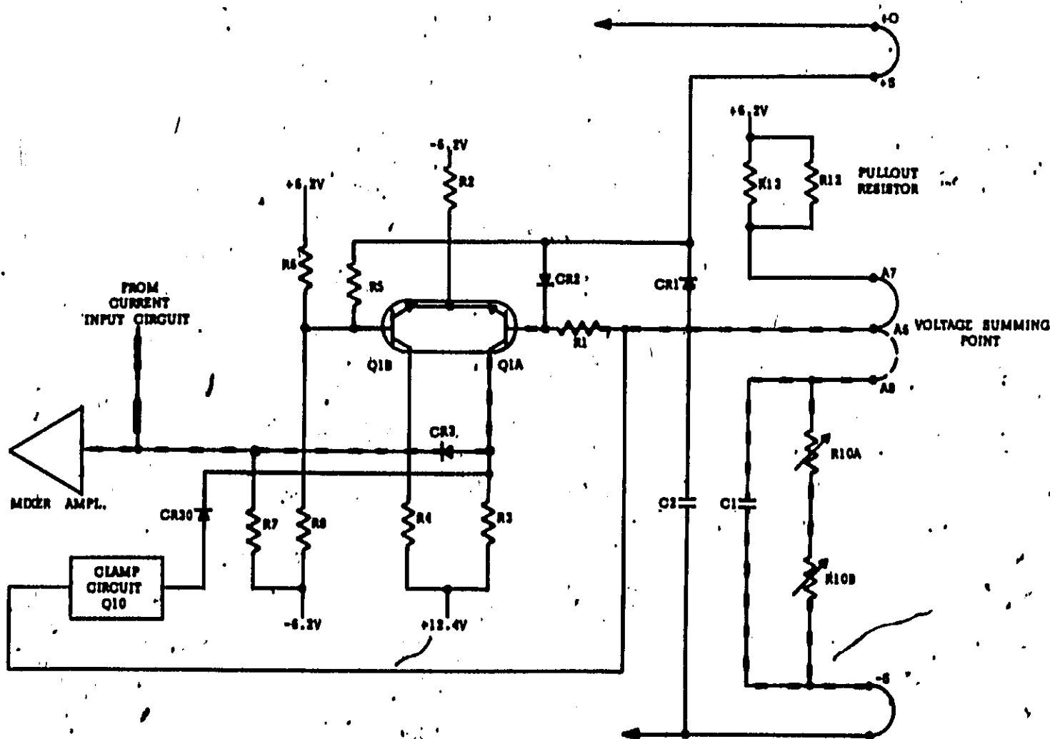
Figure 4-3. Constant Voltage Input Circuit, Simplified Schematic
