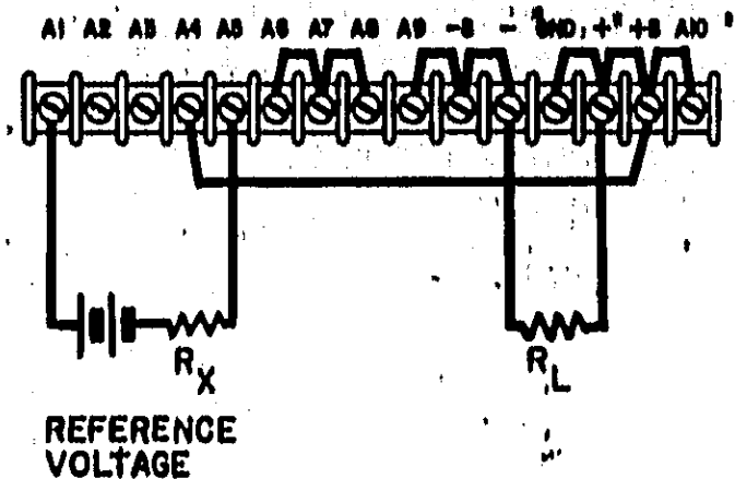
Figure 3-6. Remote Voltage Programming (Constant Current)
