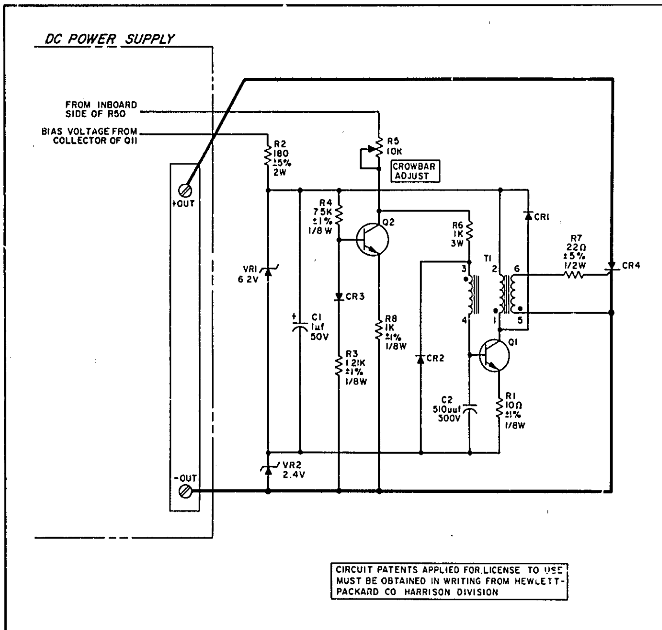
Figure A-1. Model 6113A Overvoltage Protection Crowbar
