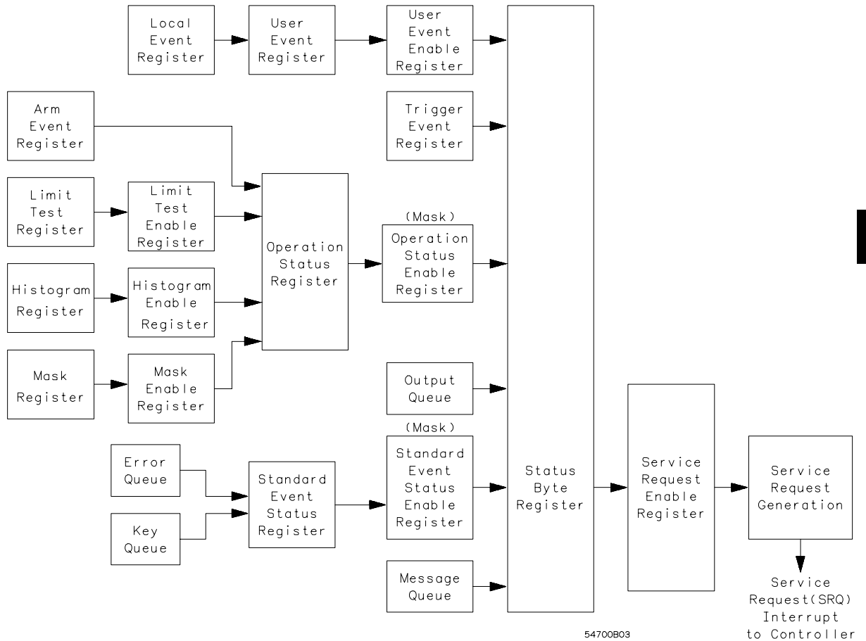
Status Reporting Overview Block Diagram
