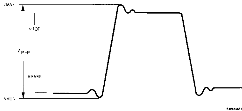
Pulse where the top and bottom are well-defined
