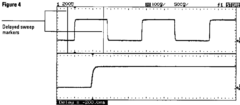
Time reference set to left
