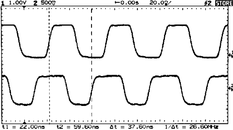
Cursors used to make channel-to-channel delay measurements
