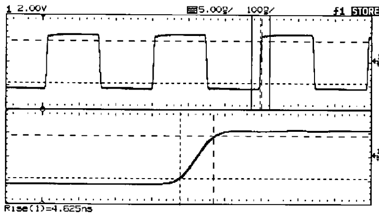
Delayed sweep isolates a leading edge for a rise time measurement
