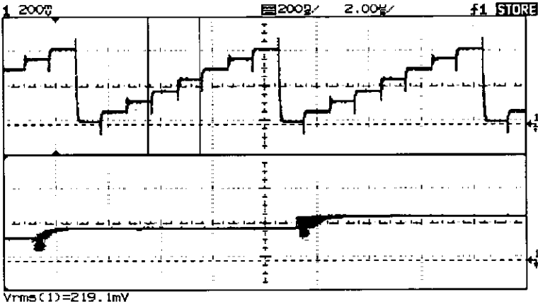
Delayed sweep isolates an area of interest for an rms voltage measurement
