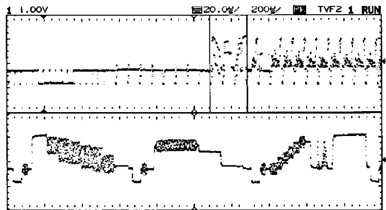
Second vertical interval windowed on the VITS
