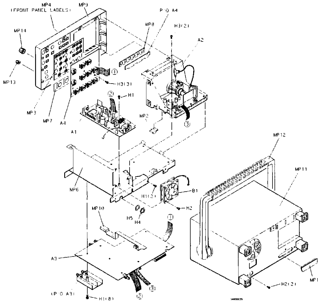
Exploded view of oscilloscope showing reference designators.
