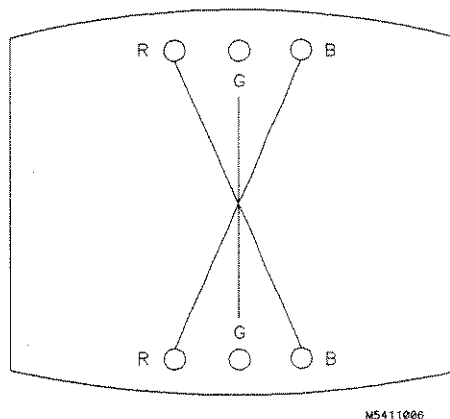
Figure 4-9. Y BOW CROSS Adjustment
