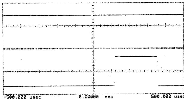
Figure 6C-34. Test Loop 28 Troubleshooting Waveform on the A/D Assembly.
