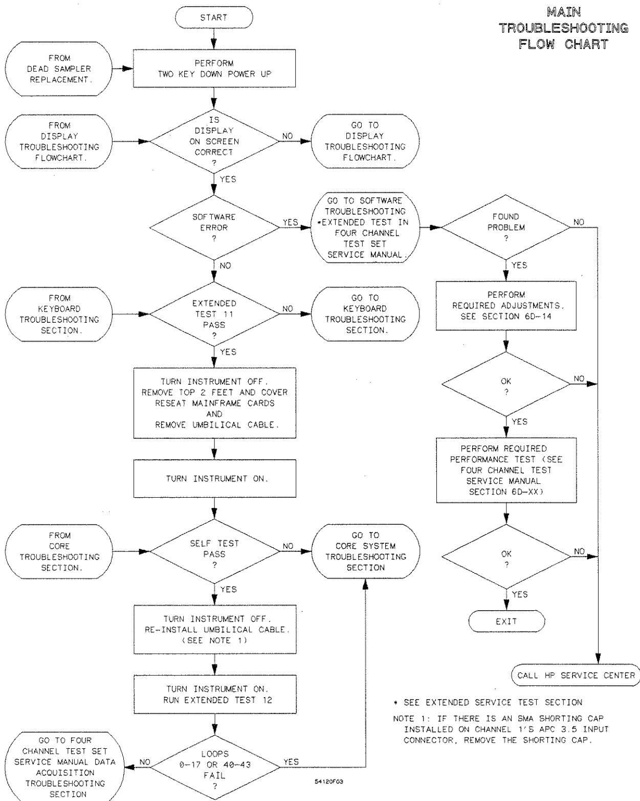
Figure 6D-1. Main Troubleshooting Flowchart
