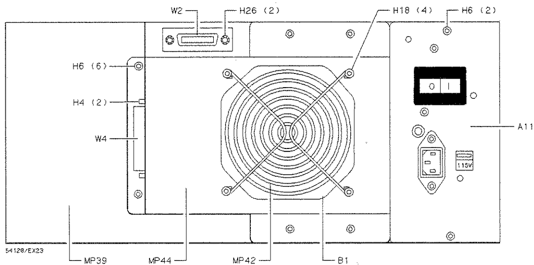
Figure 5-4. Rear Panel
