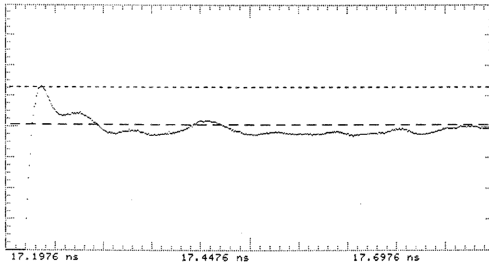
Figure 4-8. TOP Adjustment
