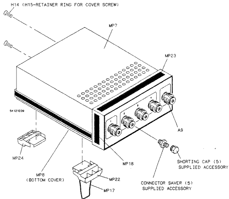
Figure 5-1. Assembled View
