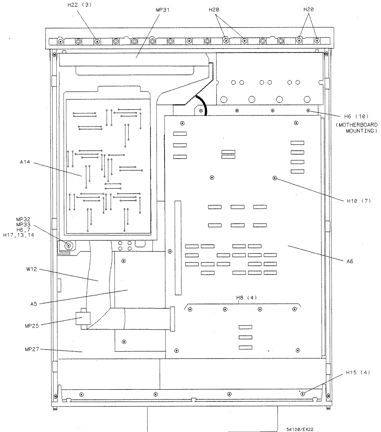
Figure 5-2. Bottom View
