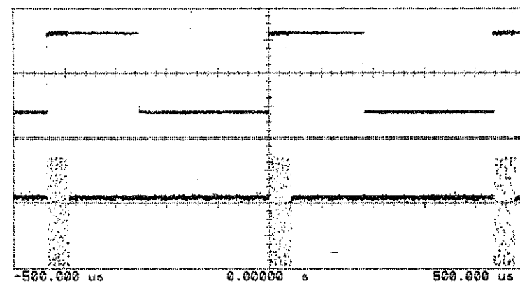
Figure 6C-15 Test Loop 20 Troubleshooting Waveform on the Horizontal Assembly
