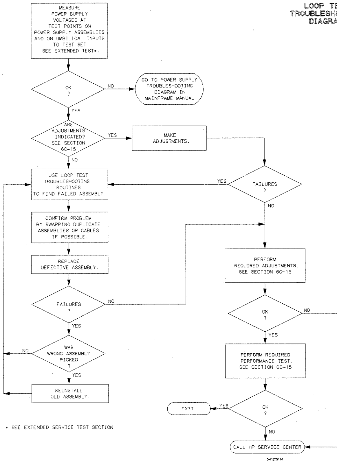
Figure 6C-5. Loop Test Troubleshooting Flowchart
