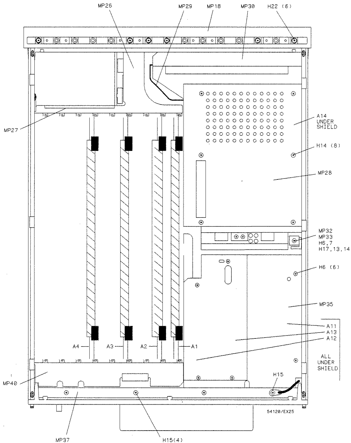
Figure 5-1. Top View
