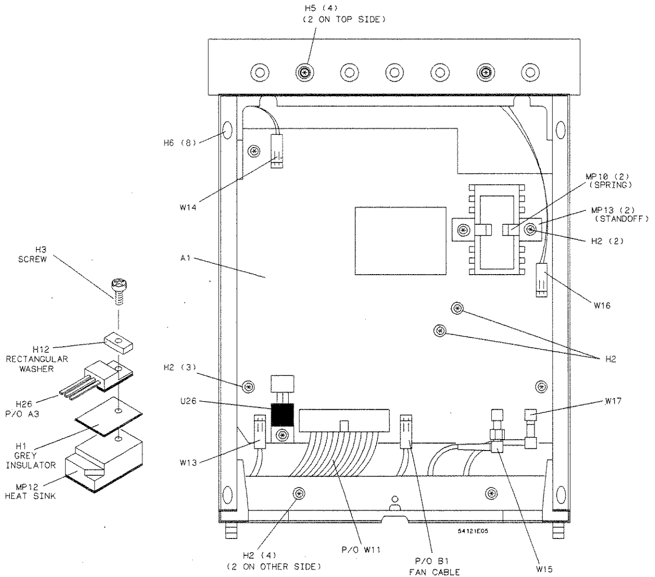
Figure 5-4. Bottom View
