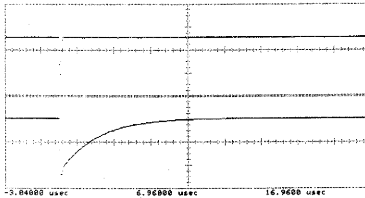
Figure 6C-59. With Pulse Filter Removed from Test Set, on the Horizontal Assembly, 2 \mu s/div.
