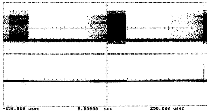
Figure 6C-60. With Pulse Filter Removed from Test Set, on the Horizontal Assembly, 50 \mu s/div.
