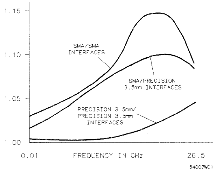
Figure 3A-2. Typical SWR of SMA and APC 3.5 Connectors
