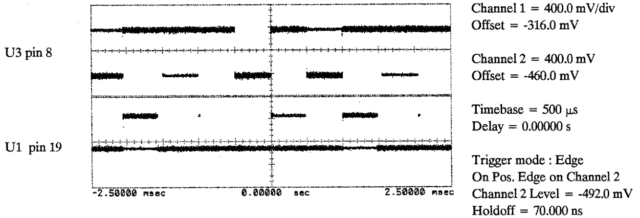
Figure 6C-28. Test Loop 26 Troubleshooting Waveform on the Horizontal Assembly.
