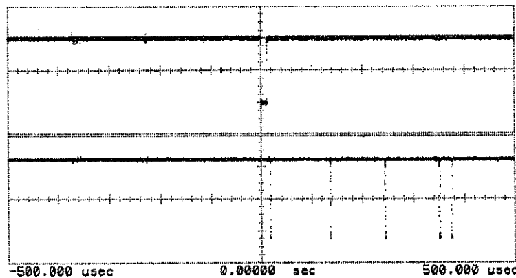
Figure 6C-32. Test Loop 28 Troubleshooting Waveform on the A/D Assembly.
