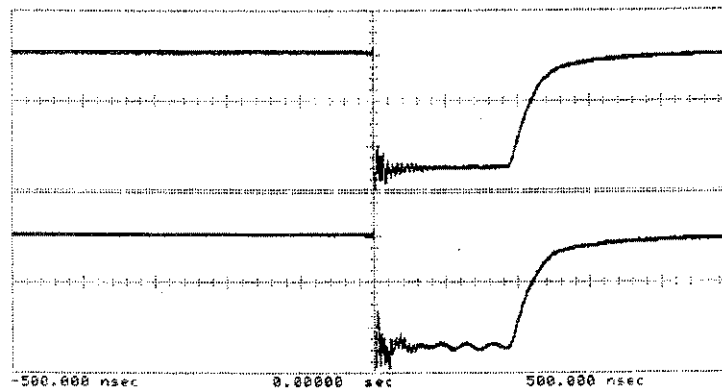
Figure 6C-61. With Pulse Filter Installed in Test Set, on the Horizontal Assembly, 100 ns/div.
