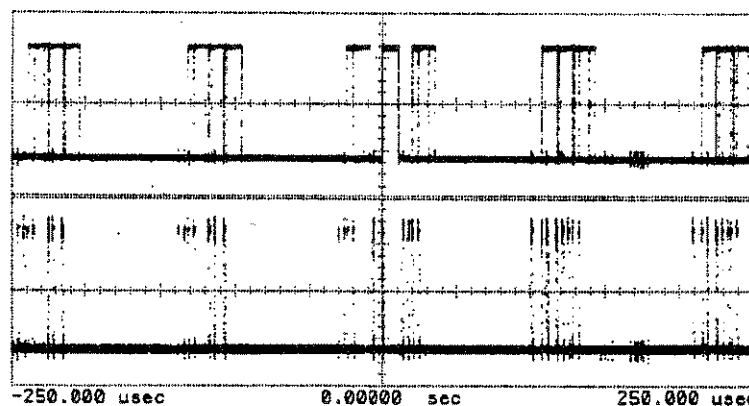
Figure 6C-33. Test Loop 28 Troubleshooting Waveform on the A/D Assembly.
