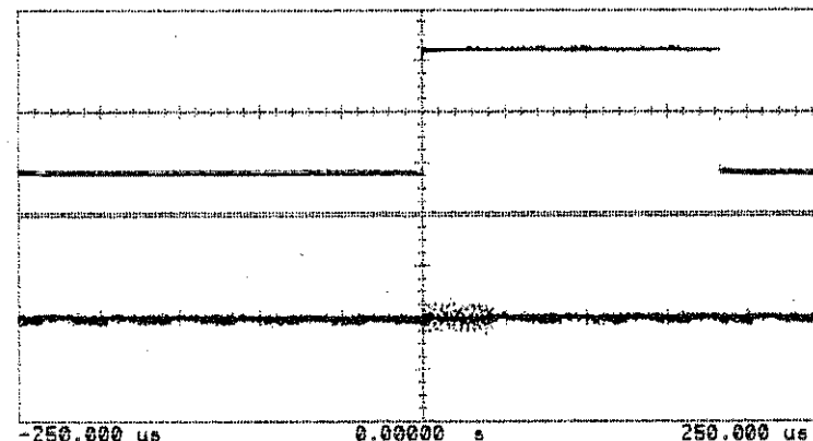
Figure 6C-14. Test Loop 20 Troubleshooting Waveform on the Horizontal Assembly
