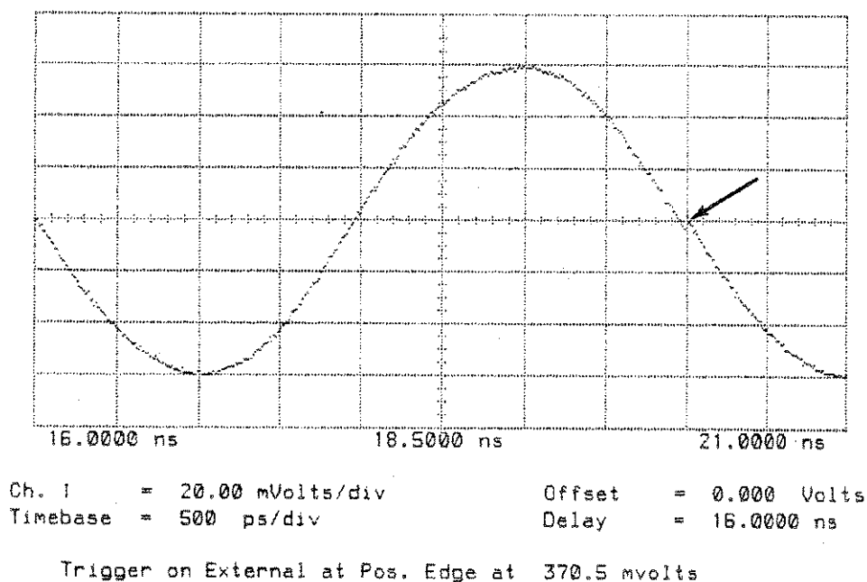
Figure 4-1. Trace Discontinuity at Eighth Graticule
