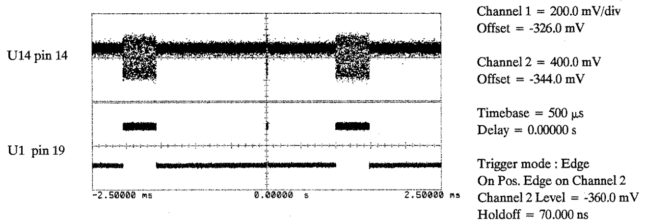
Figure 6C-30. Test Loop 26 Troubleshooting Waveform on the Horizontal Assembly.
