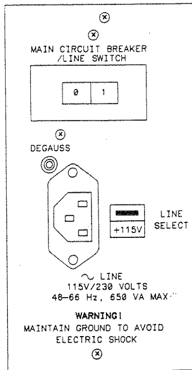
Figure 4-2. Power Module
