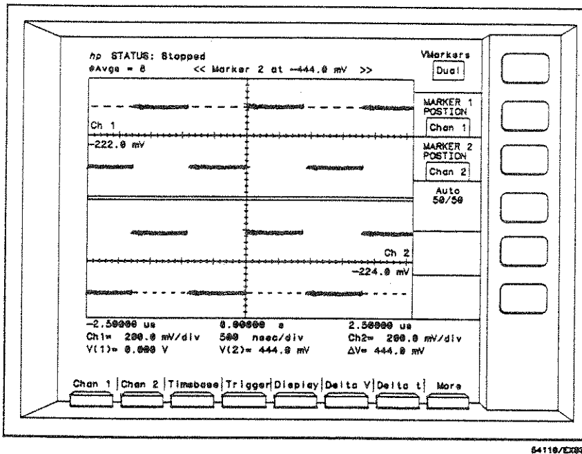
Figure 7-6. Delta V markers on Split Screen.
