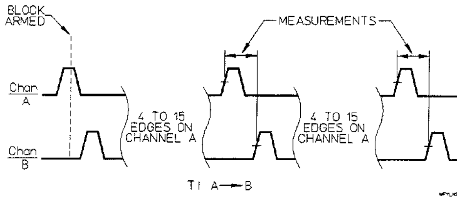
Figure 1-23. Time Interval | Random Sampling
