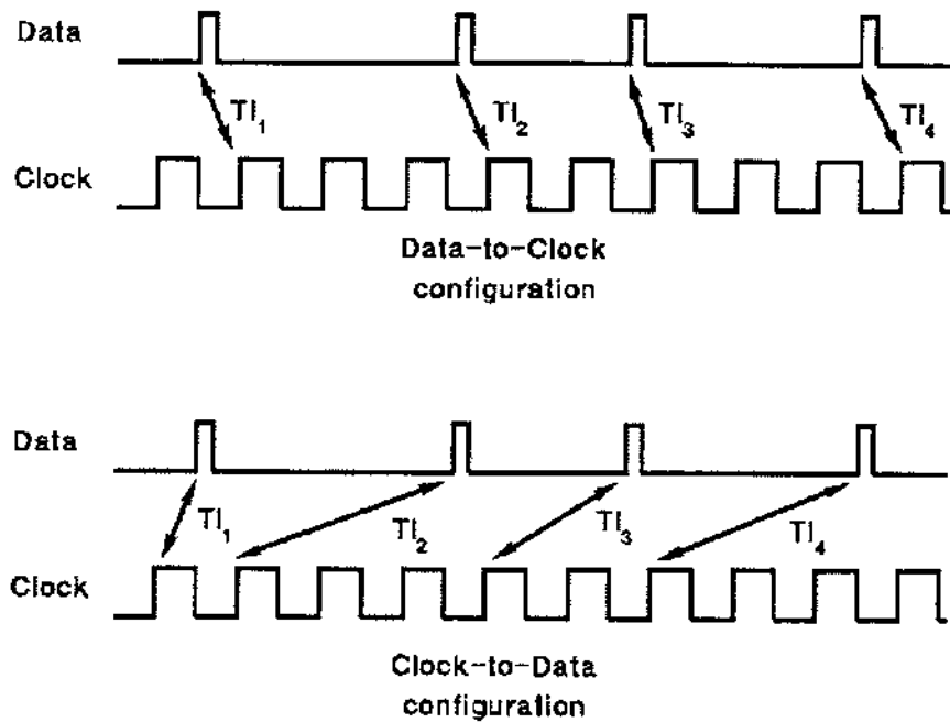
Figure 4-21. It is recommended that the time interval measurement start on the data channel and stop on the clock channel. This will result in a single histogram distribution.
