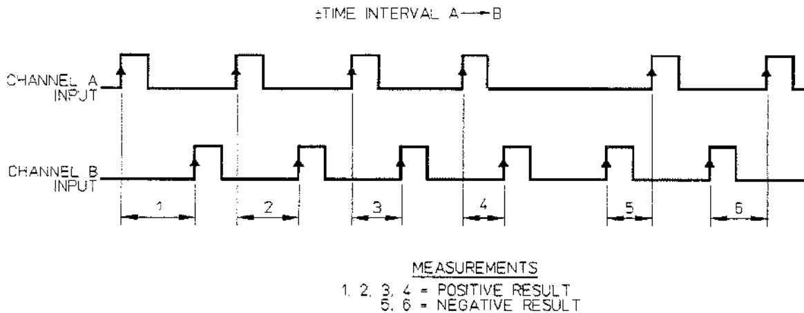
Figure 1-7. \pm Time Interval on Two Channels
