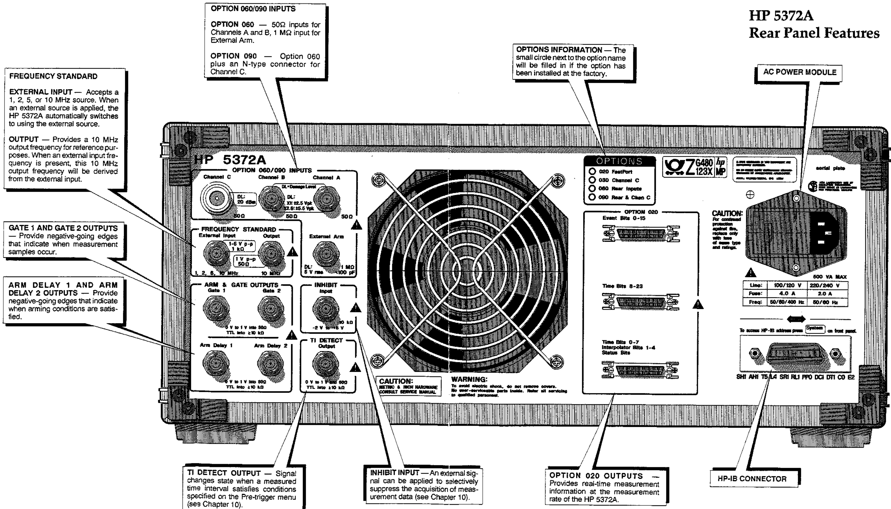
Figure 6-2. Rear Panel Features
