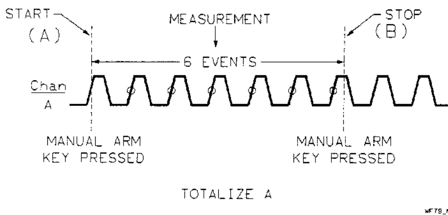
Figure 5-58. MANUAL Timing Diagram
