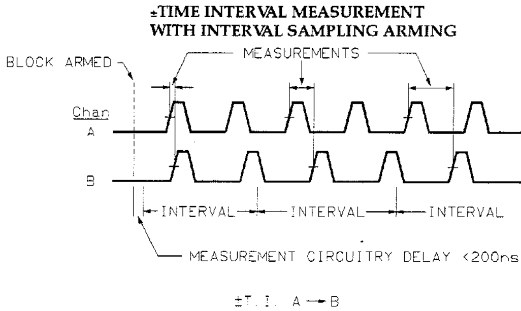
Figure 1-35. ± Time Interval | Interval Sampling
