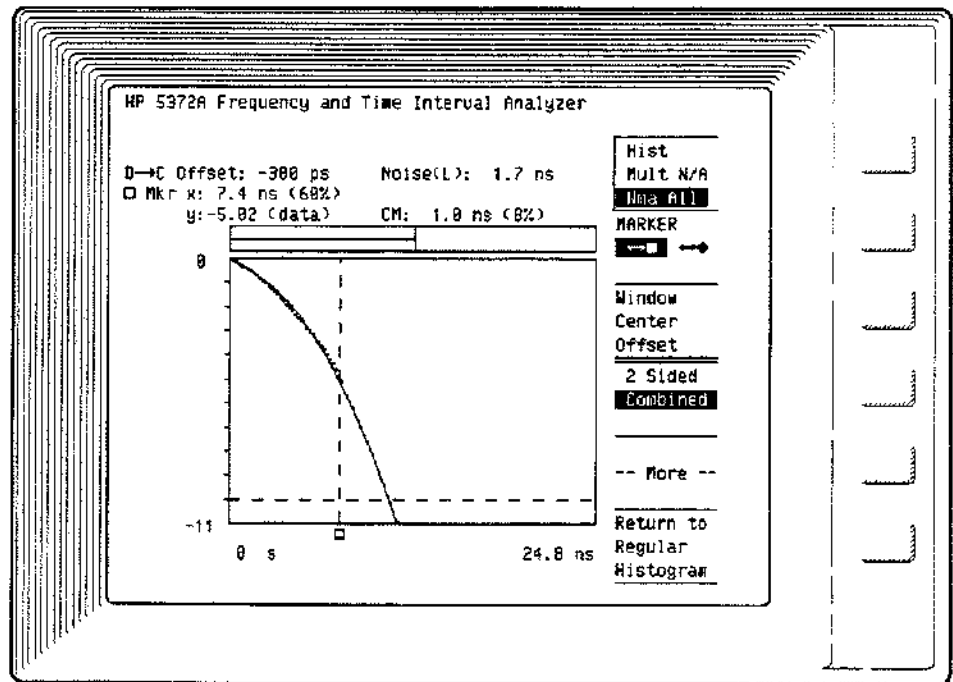
Figure 4-26. Data-to-clock margin information can be viewed in the combined mode.
