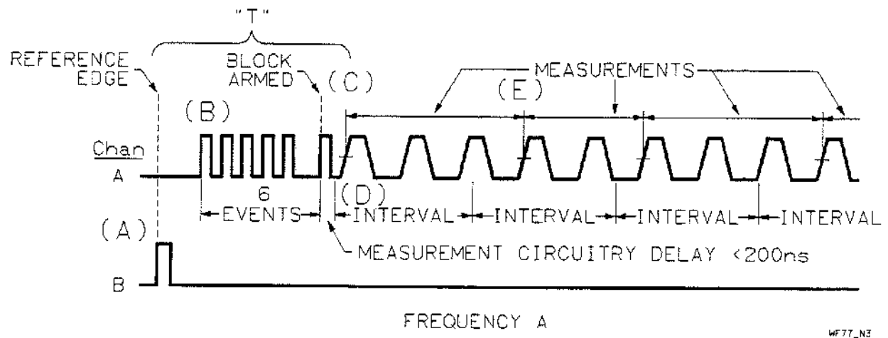
Figure 5-52. EVENT/INTERVAL Timing Diagram
