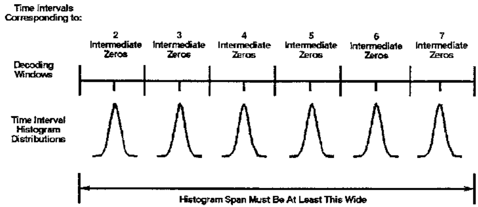
Figure 4-27. It is necessary to configure the histogram measurement with a wide enough span to cover all valid interval values for proper margin analysis.
