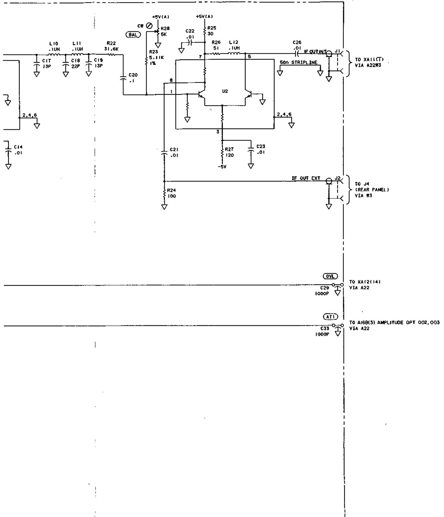
Figure 8-45. A25 Preamp Assembly
