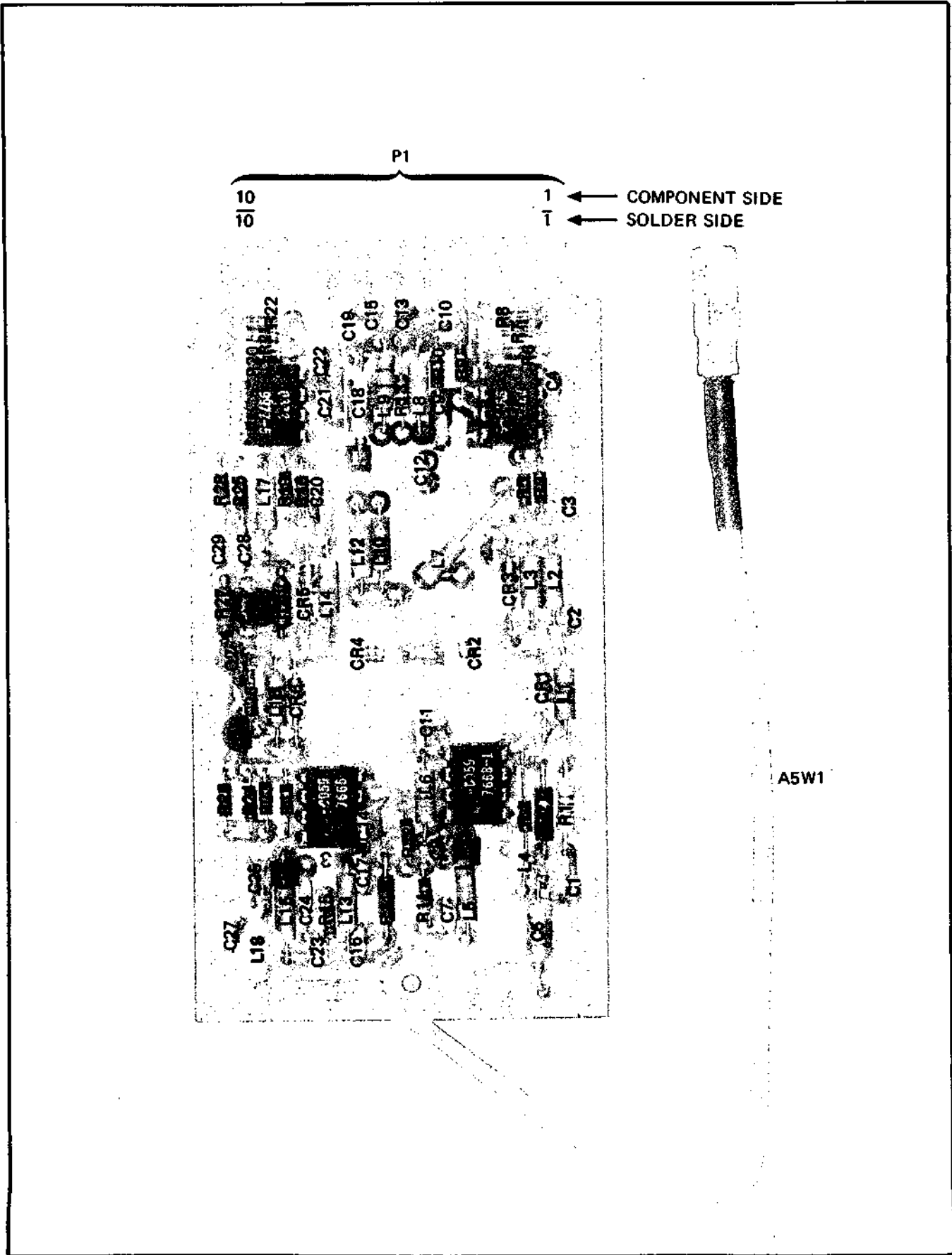
Part of Figure 8-28. A5 RF Multiplexer Assembly
