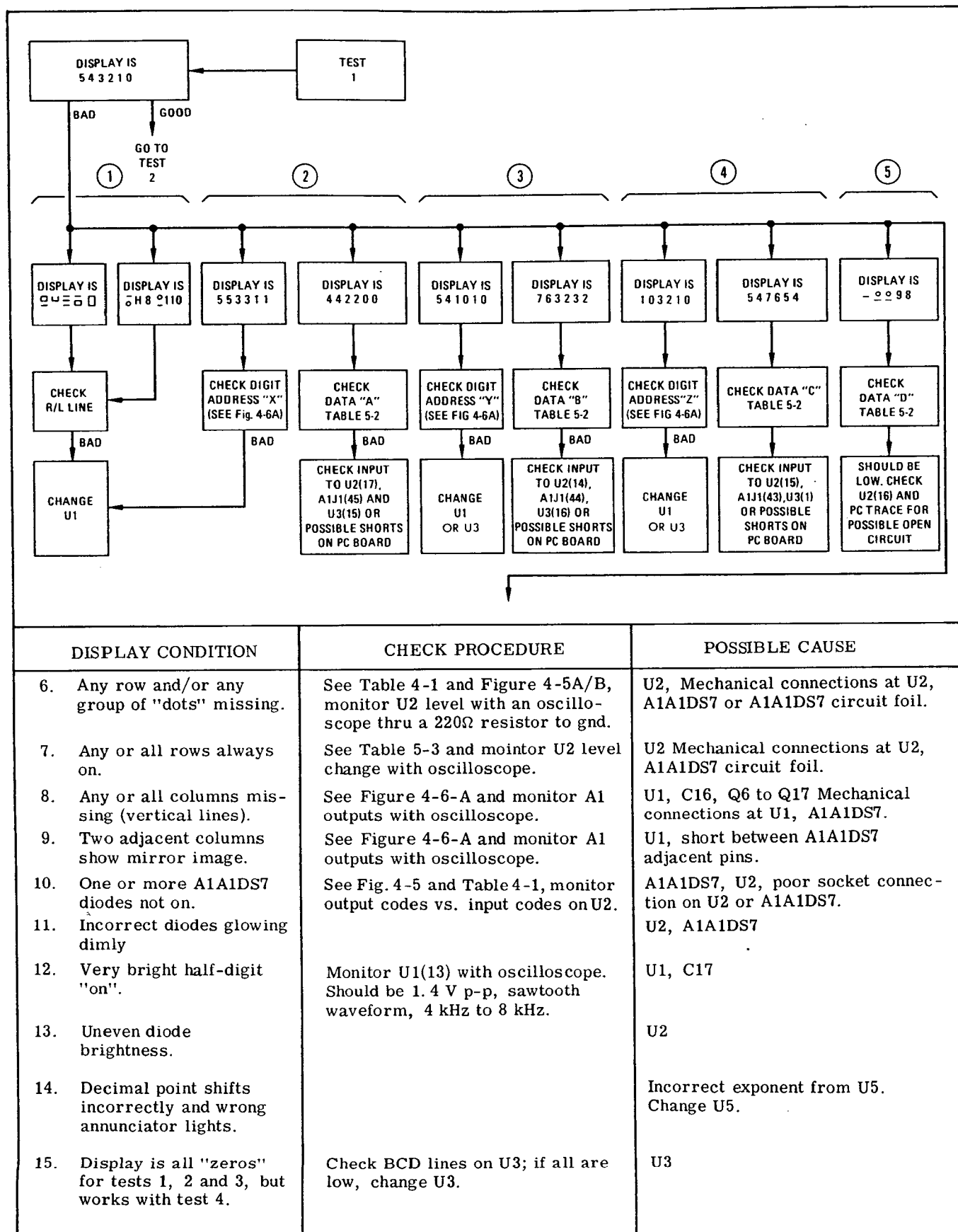
Figure 5-3A. Display Checks
