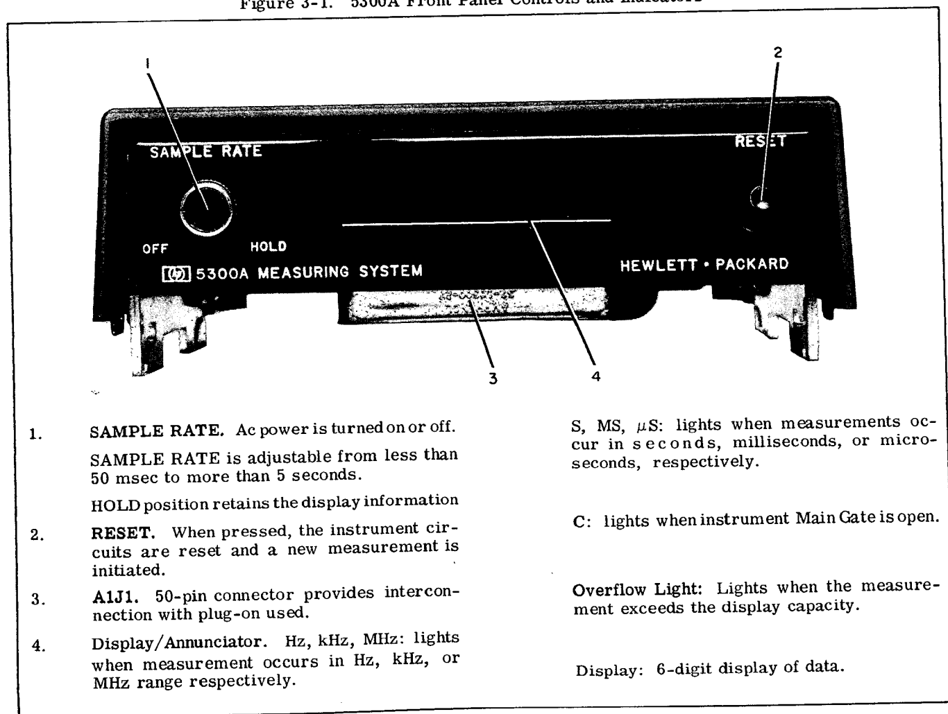
Figure 3-1. 5300A Front Panel Controls and Indicators
