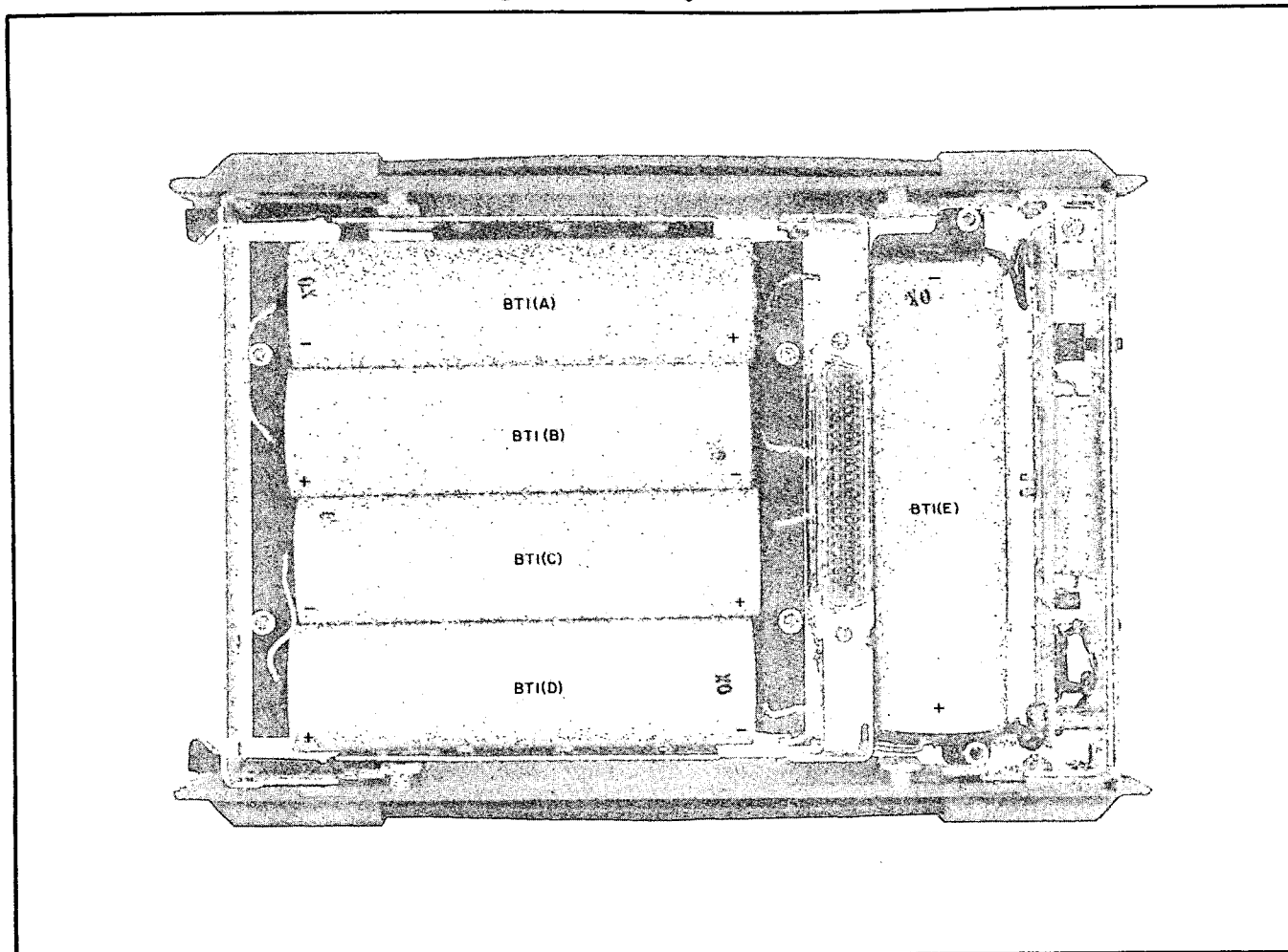
Figure 5-5. Battery Removal
