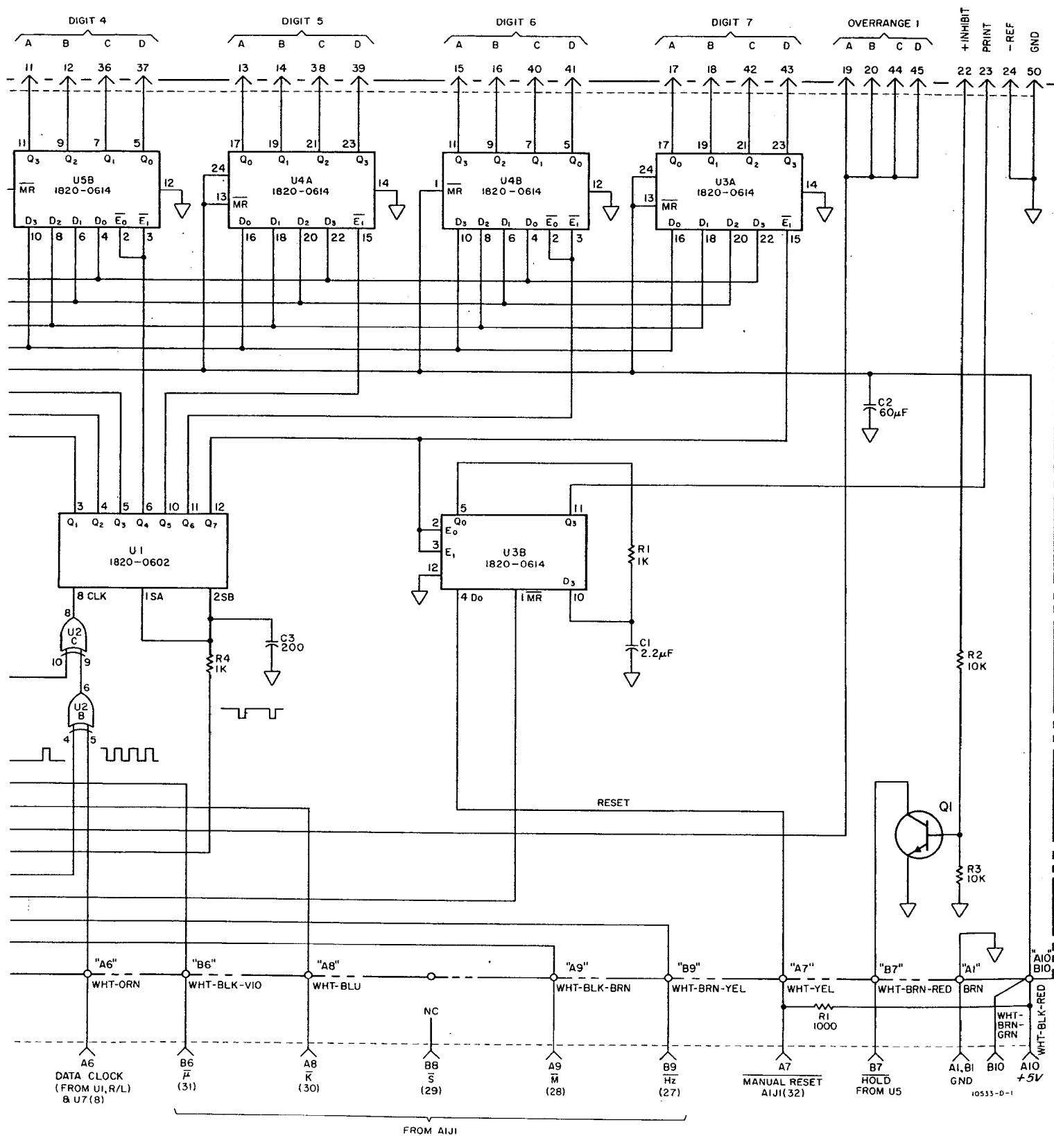
Figure 8-4 10533A Digital Recorder Interface (Available as Accessory Only)
