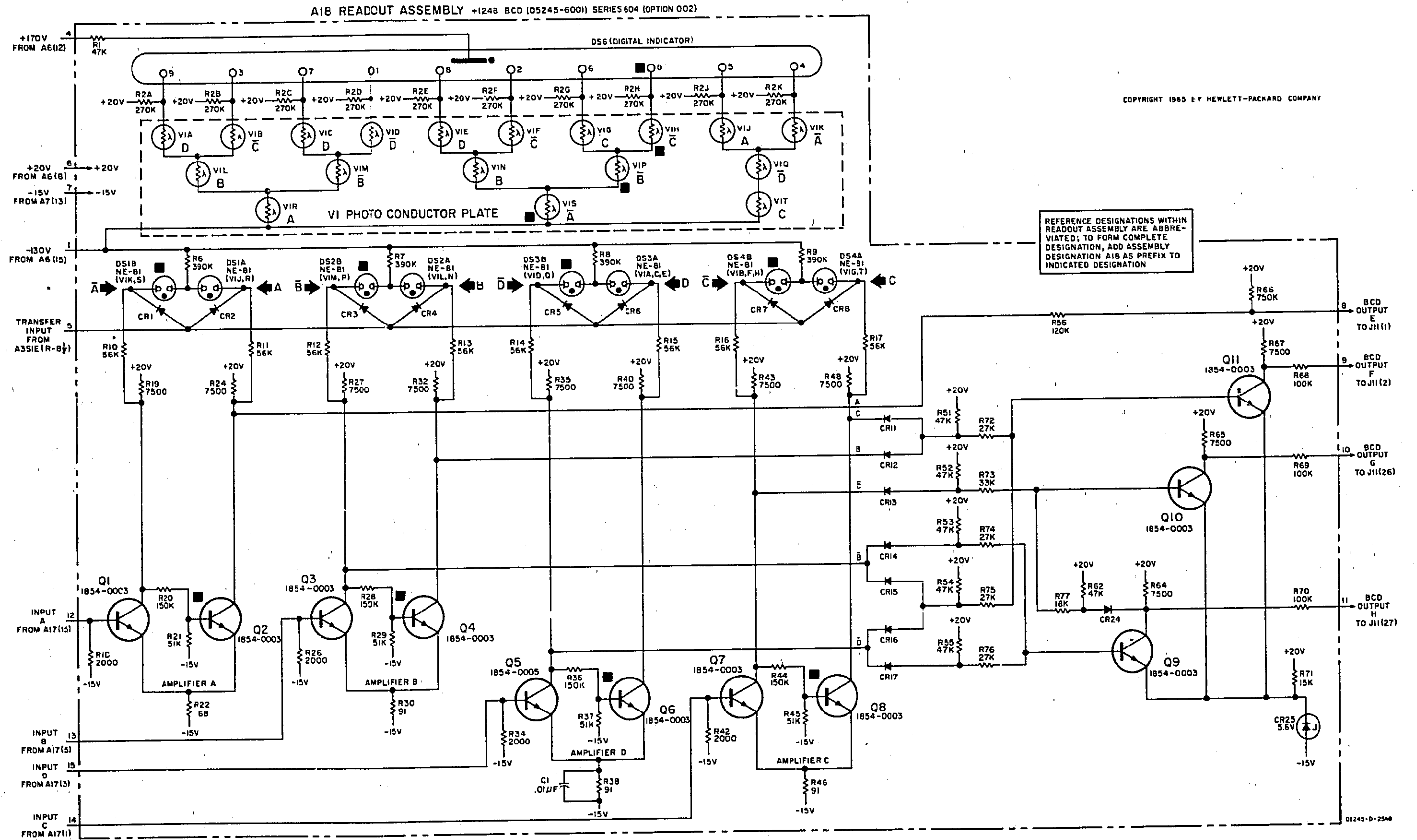
Figure 7-15. A18 Readout (05245-6001) Option 002
