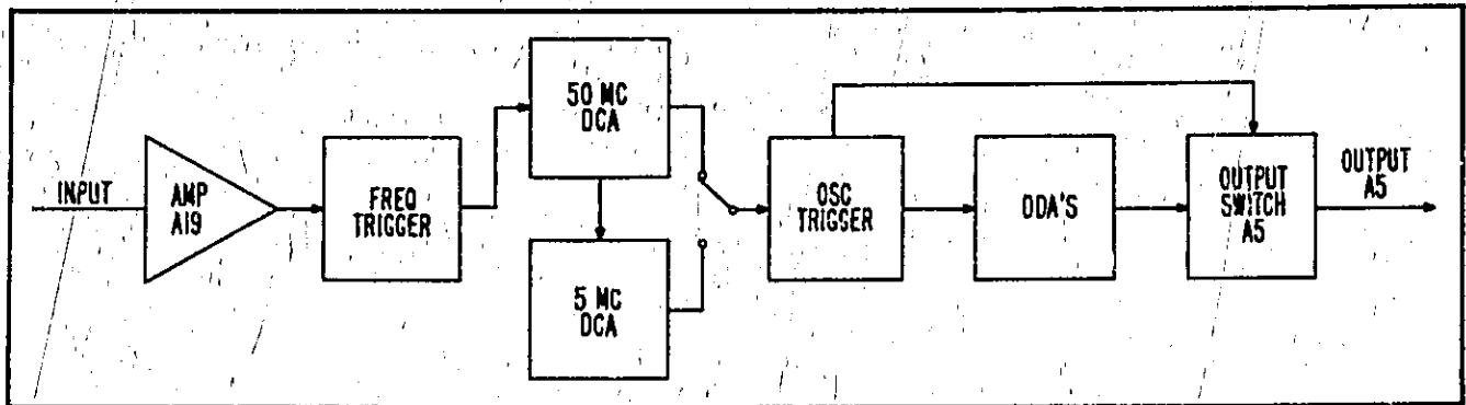
Figure 2-11. Scaler Operation
