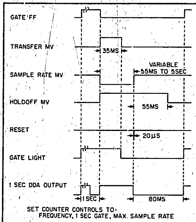
Figure 2-12. Time Sequence
