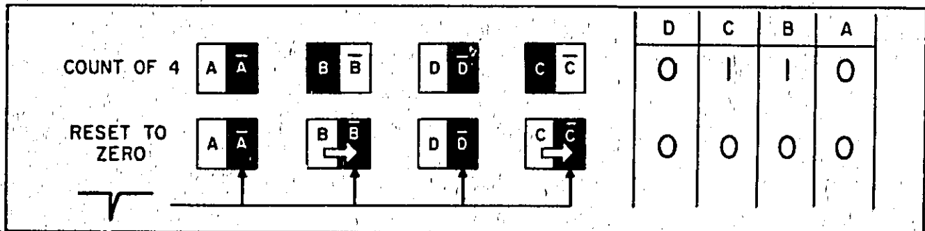
Figure 2-7. Typical Reset Operation in Four-Binary Decimal Counter Assembly
