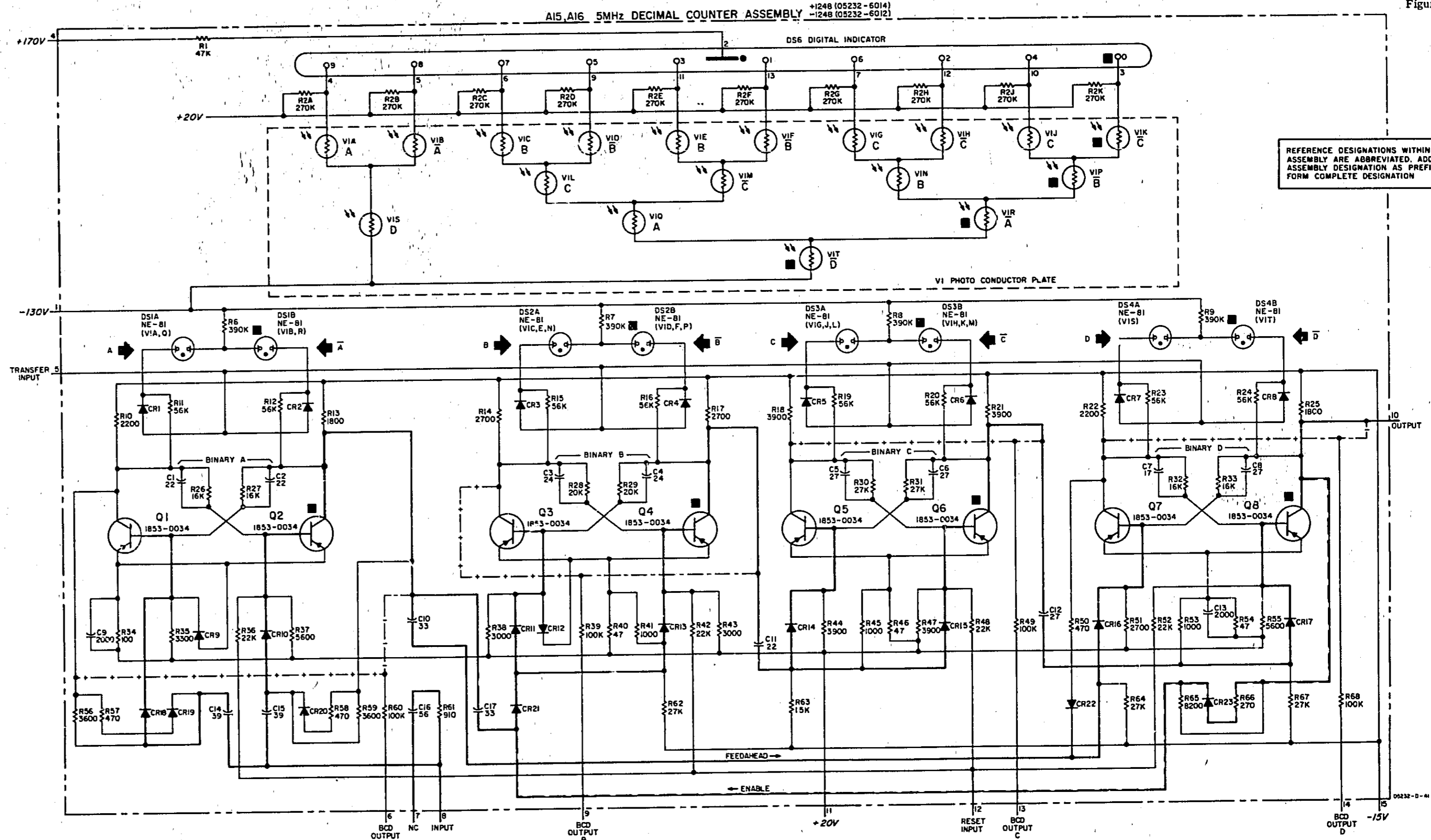
Figure 7-12. A15, A16 Decimal Counter (05232-6014, 6012) Option 002, 003
