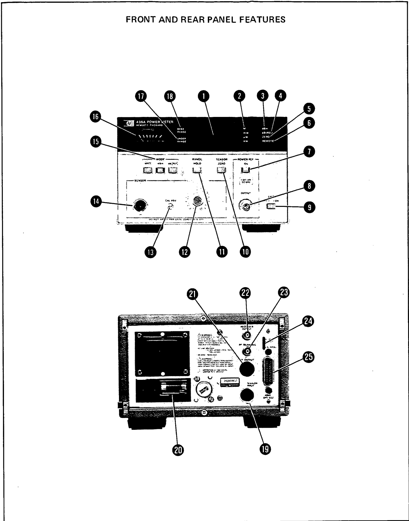
Figure 3-1. Front and Rear Panel Controls, Connectors, and Indicators (3 of 4)
