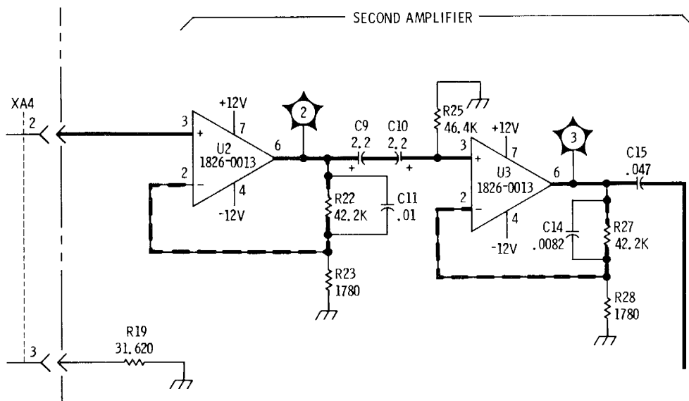
Figure 7-2. P/O A4 Assembly Schematic (Part of Change A)
