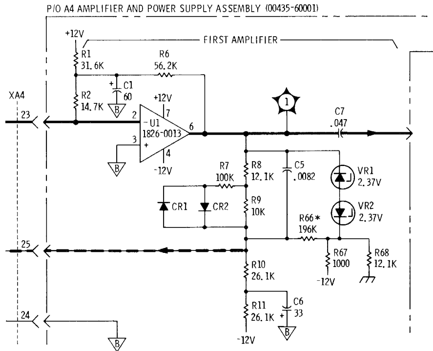
Figure 7-1. P/O A4 Assembly Schematic (Part of Change A)
