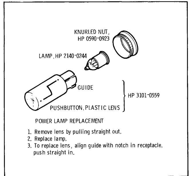
Figure 3-1. Line Switch Lamp Replacement
