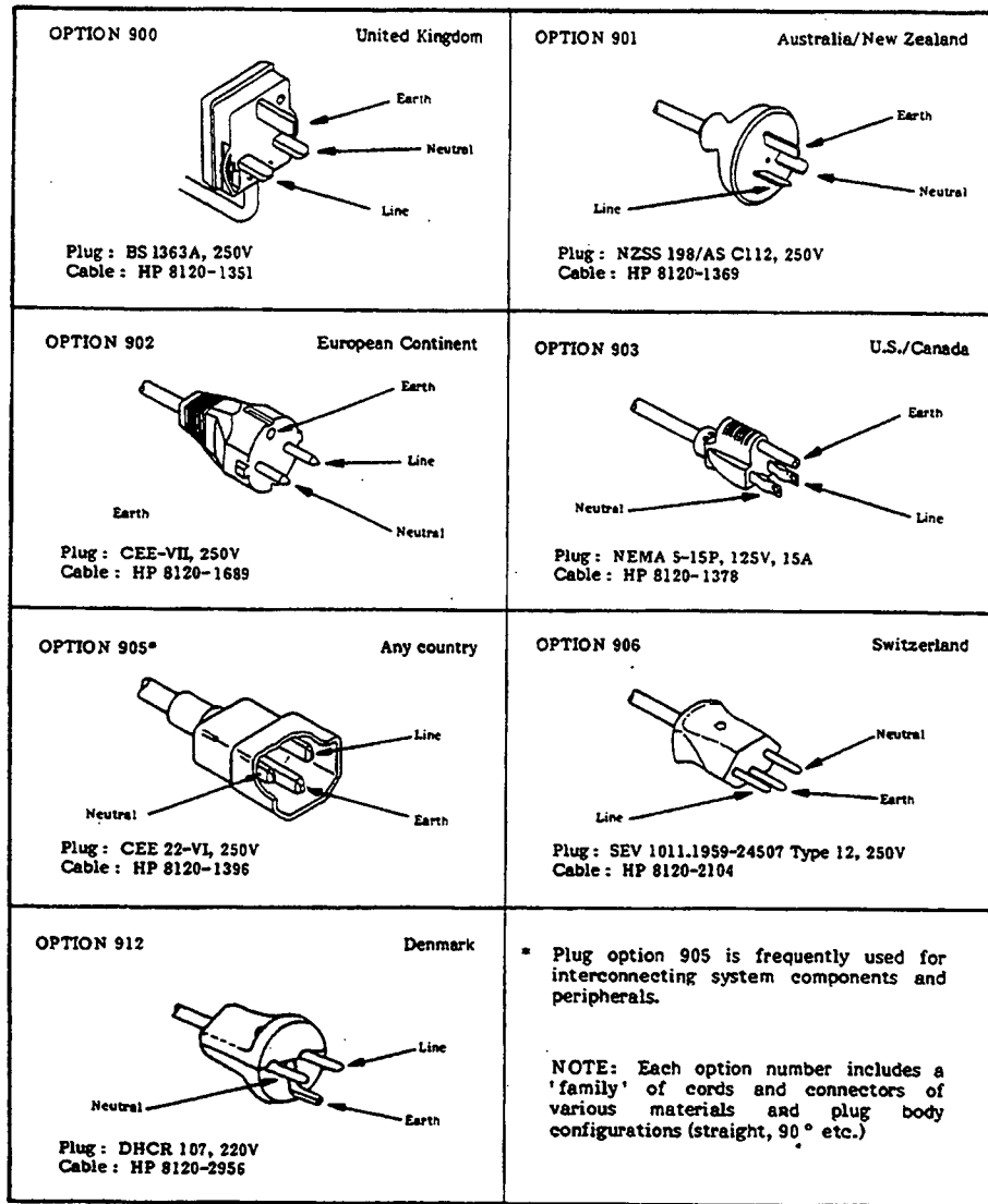
Figure 2-2. Power Cables Supplied
