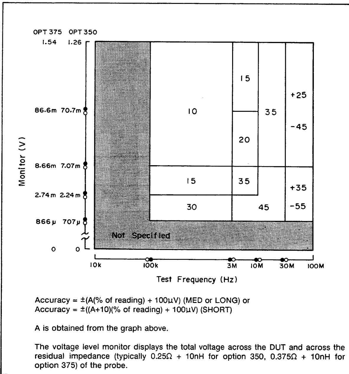
Figure 1-6. HP 41941B Voltage Monitor Accuracy
