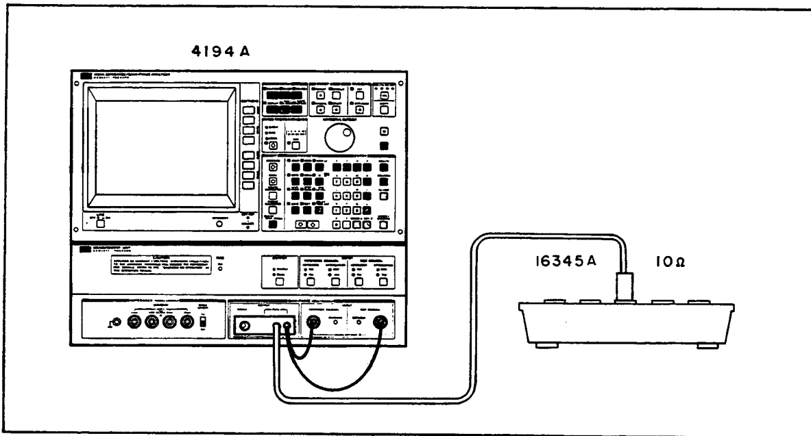
Figure 4-1. Impedance Measurement Accuracy Test Setup
