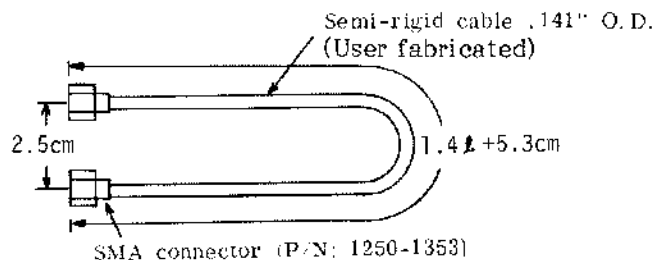
SMA connector (P/N: 1250-1353) Semi-rigid cable E/L compensator.
