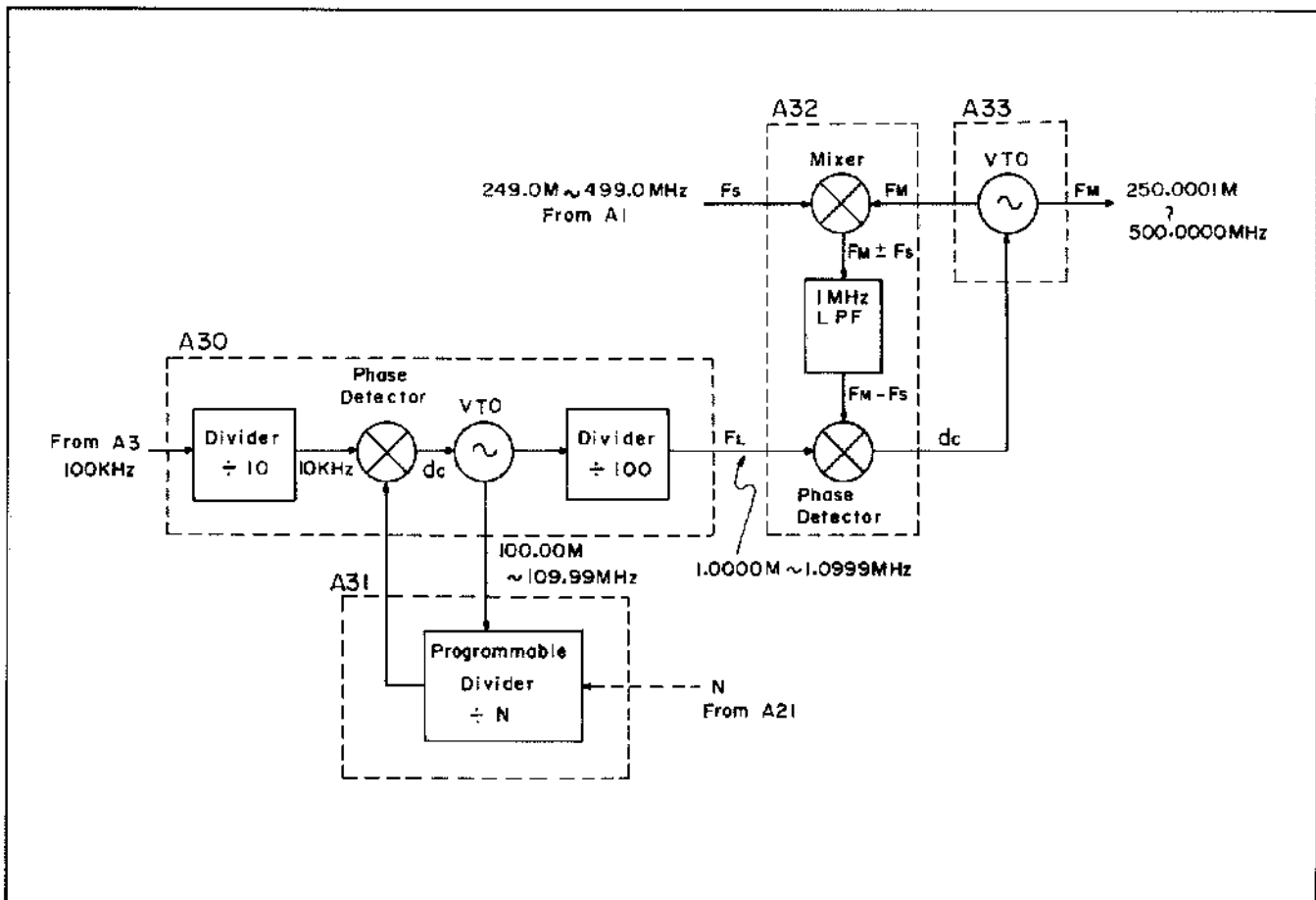
Figure 8-6. Option 002 Circuit Basic Block Diagram.
