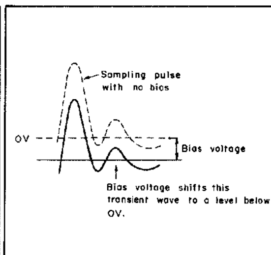
Figure 8-46. Sampling Pulse Waveform.
