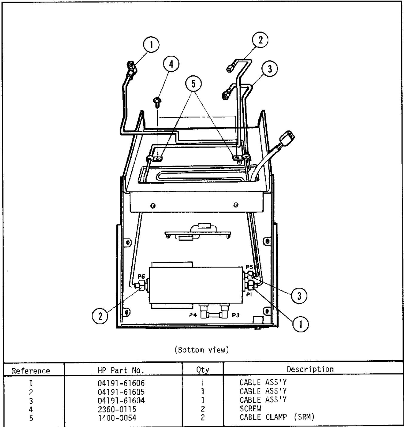
Figure 6-3. Cable Assemblies of the Directional Bridge Assembly - Exploded View.
