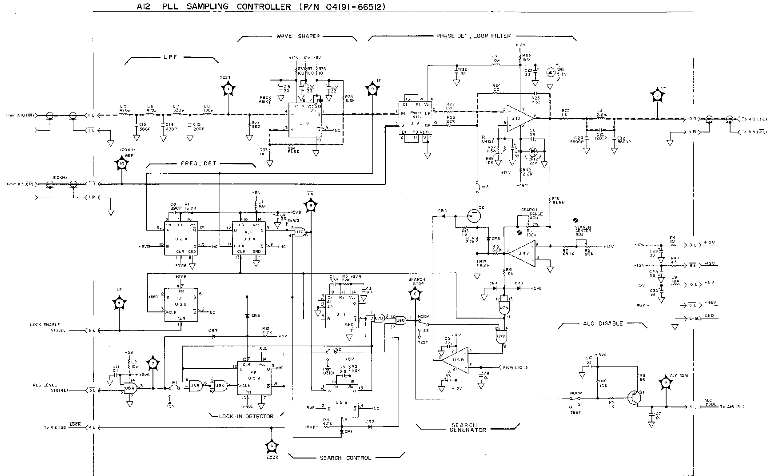
Figure 8-54. A12 PLL Sampling Controller Board Assembly Schematic Diagram.
