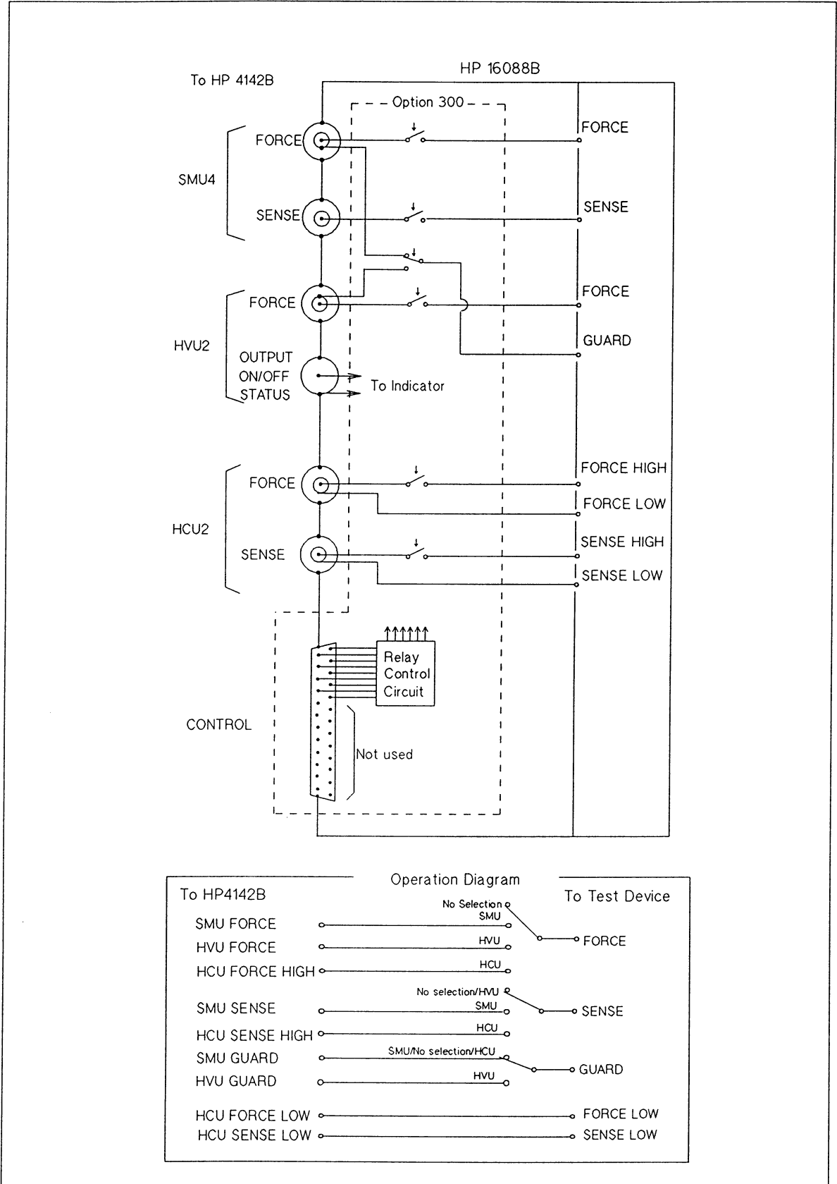
Module Selector Circuit Diagram
