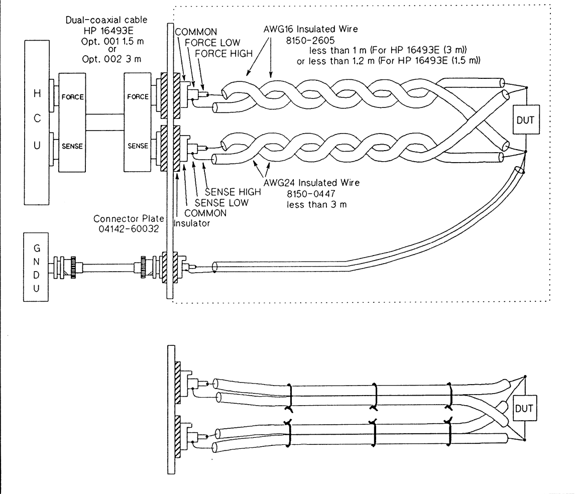
HCU Example Connection (2 of 2)
