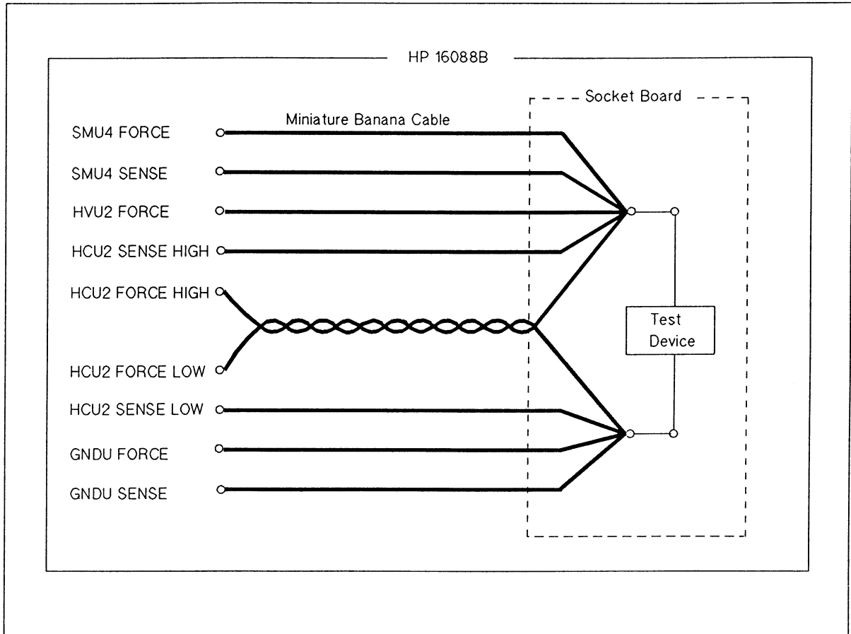
Module Selector Connections
