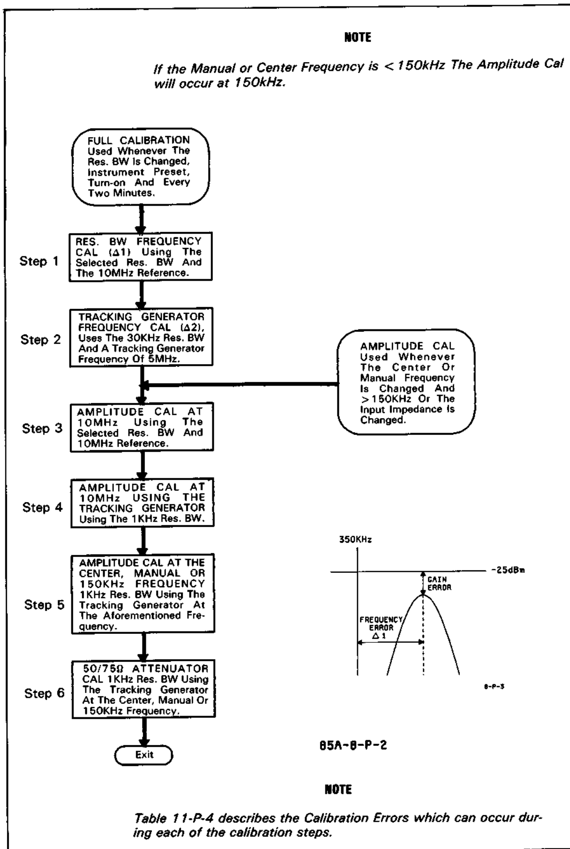
Figure 11-P-2. Calibration Sequence Flowchart
