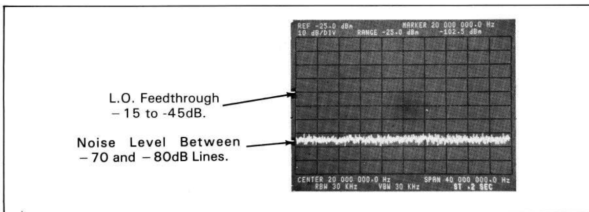
Figure 11-P-12. Correct Graphic Display
