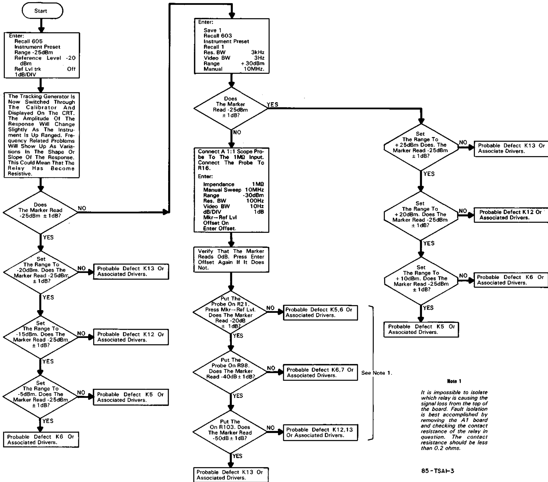
A1 Terminated Input Attenuator Troubleshooting Tree 11-43/11-44
