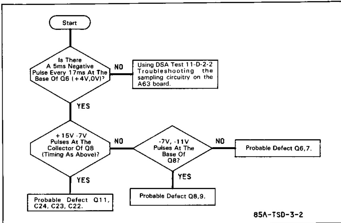
A64 Sampling Troubleshooting Tree
