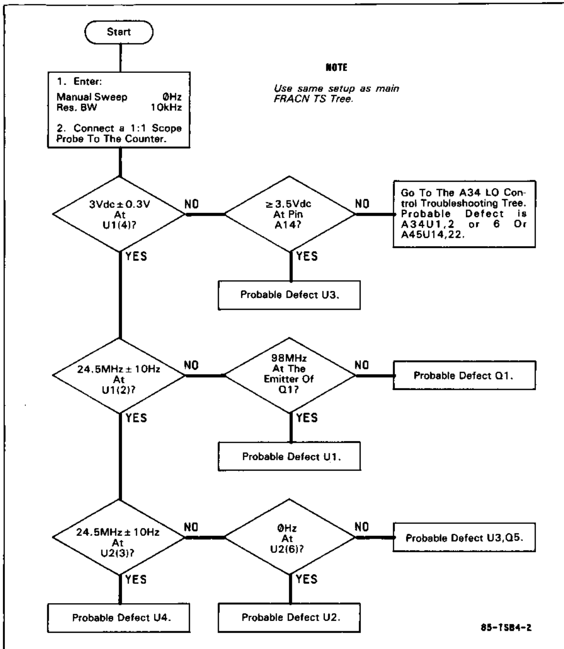
A31 Divide By 4 Troubleshooting Tree.
