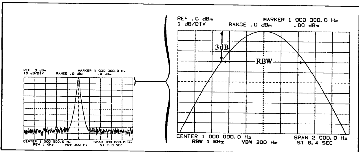
Resolution Bandwidth
