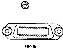
HP-IB Connector: Used to interface the instrument with the Hewlett-Packard Interface Bus (HP-IB) for remote operation. Remote operation is described in Section III, Part 2.
