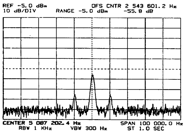
Second Harmonic
