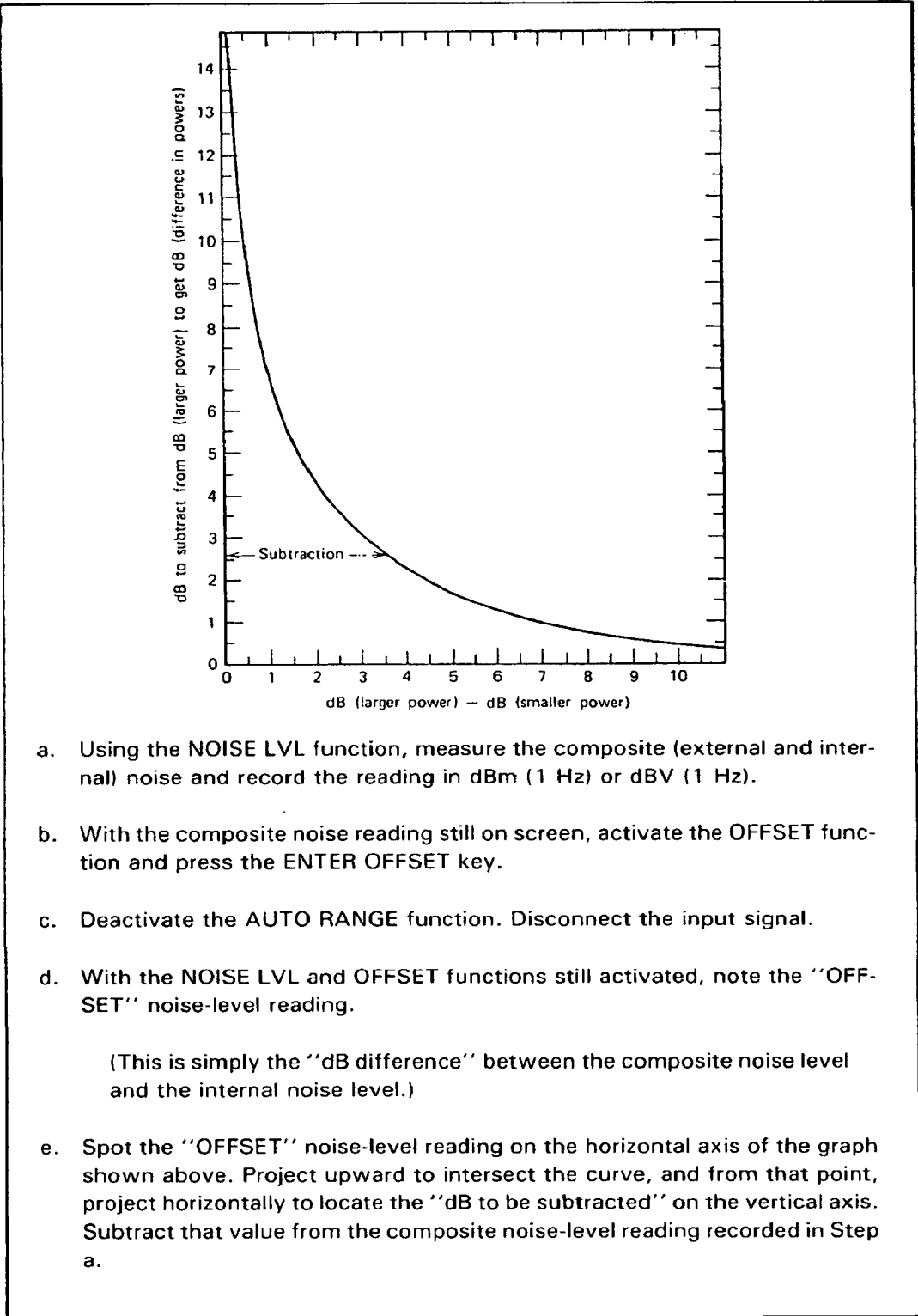
Figure C. Subtracting the Analyzer's Internal Noise
