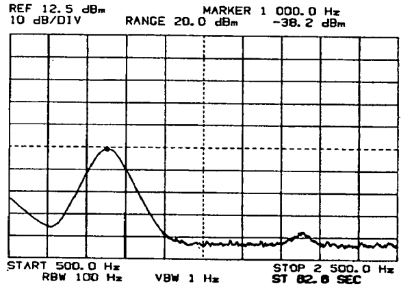
Second and Fourth-Order IM Distortion Products.
