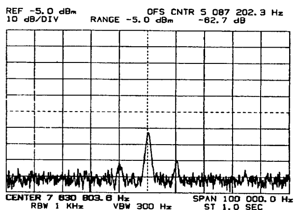
Third Harmonic
