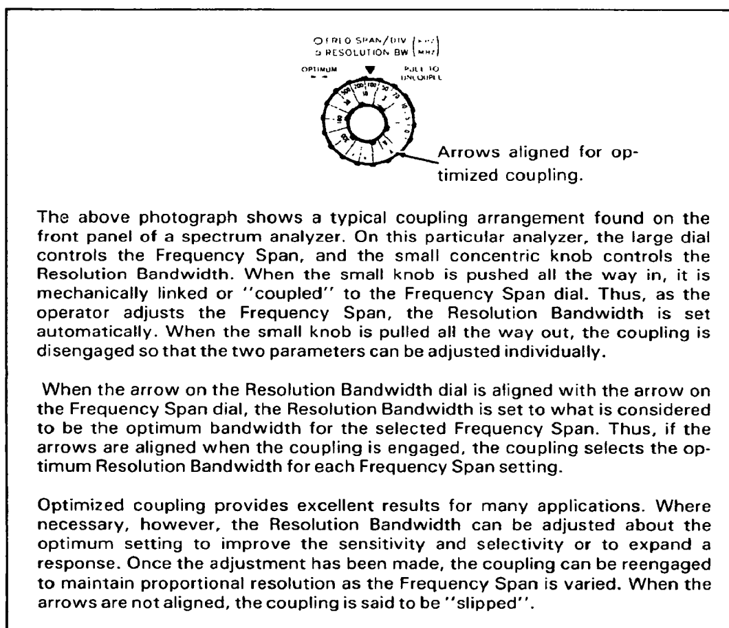
Figure 1. Mechanical Coupling.
