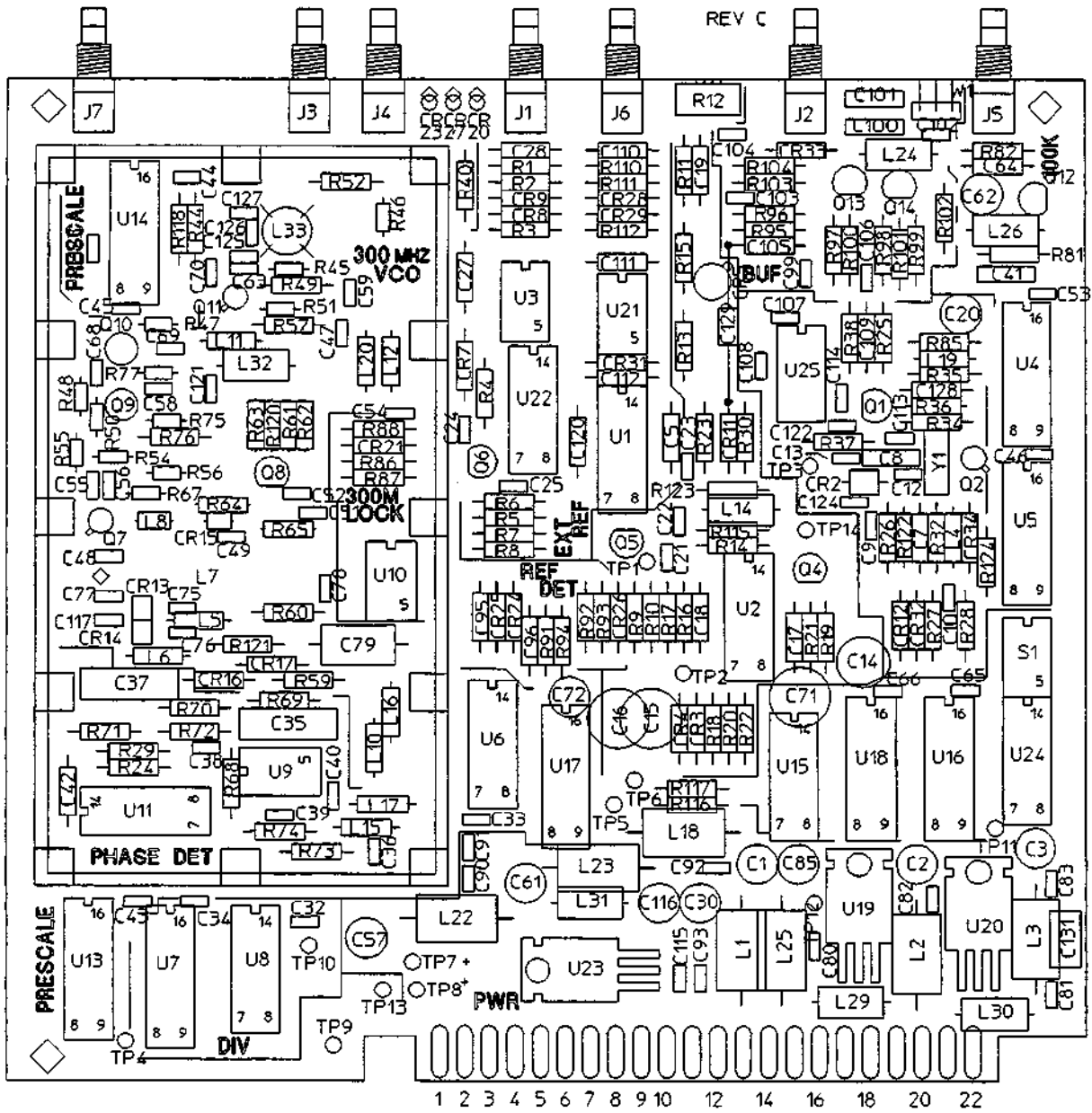
Figure 9-8. A6 Component Locator
