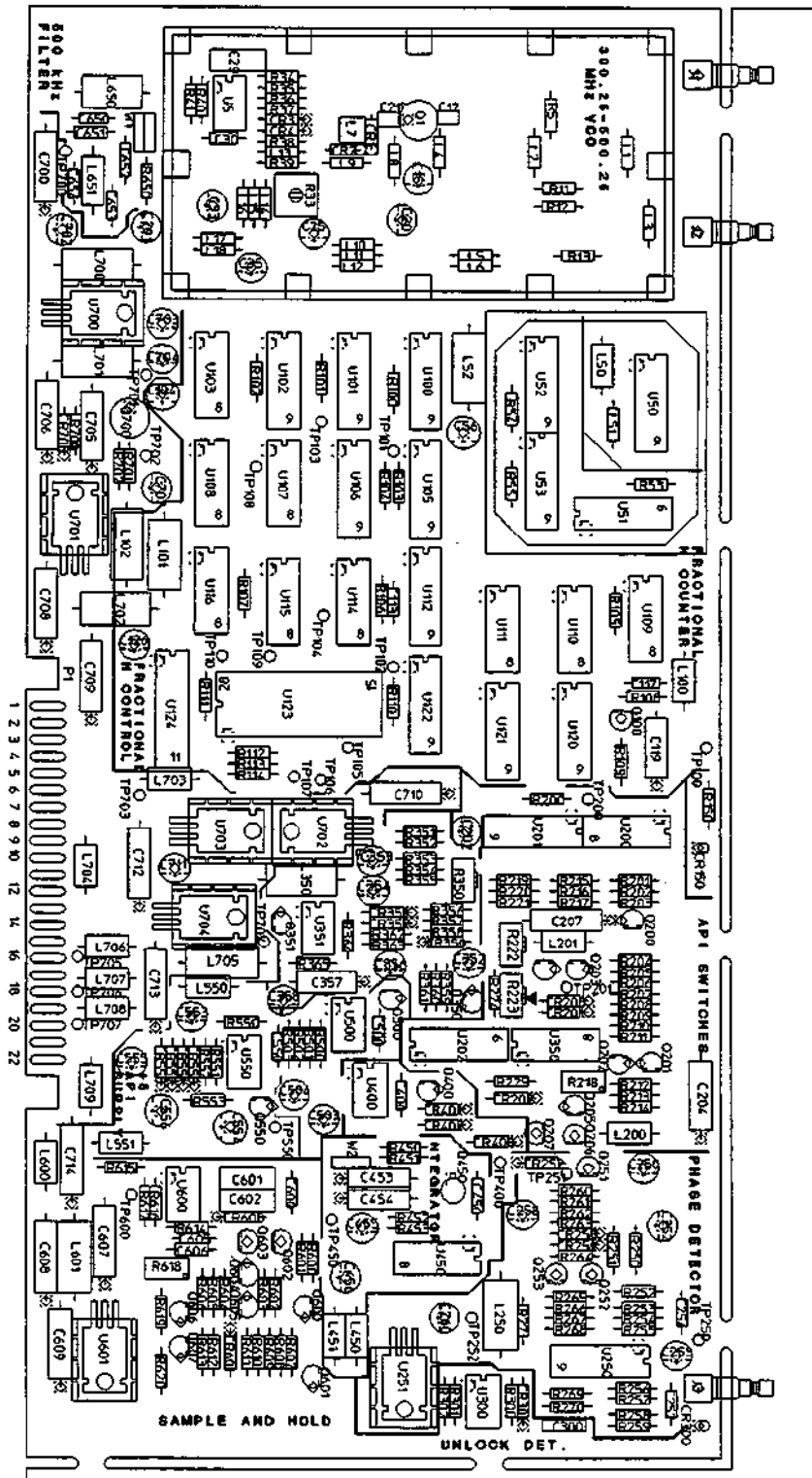
Figure 9-12. A17 Component Locator
