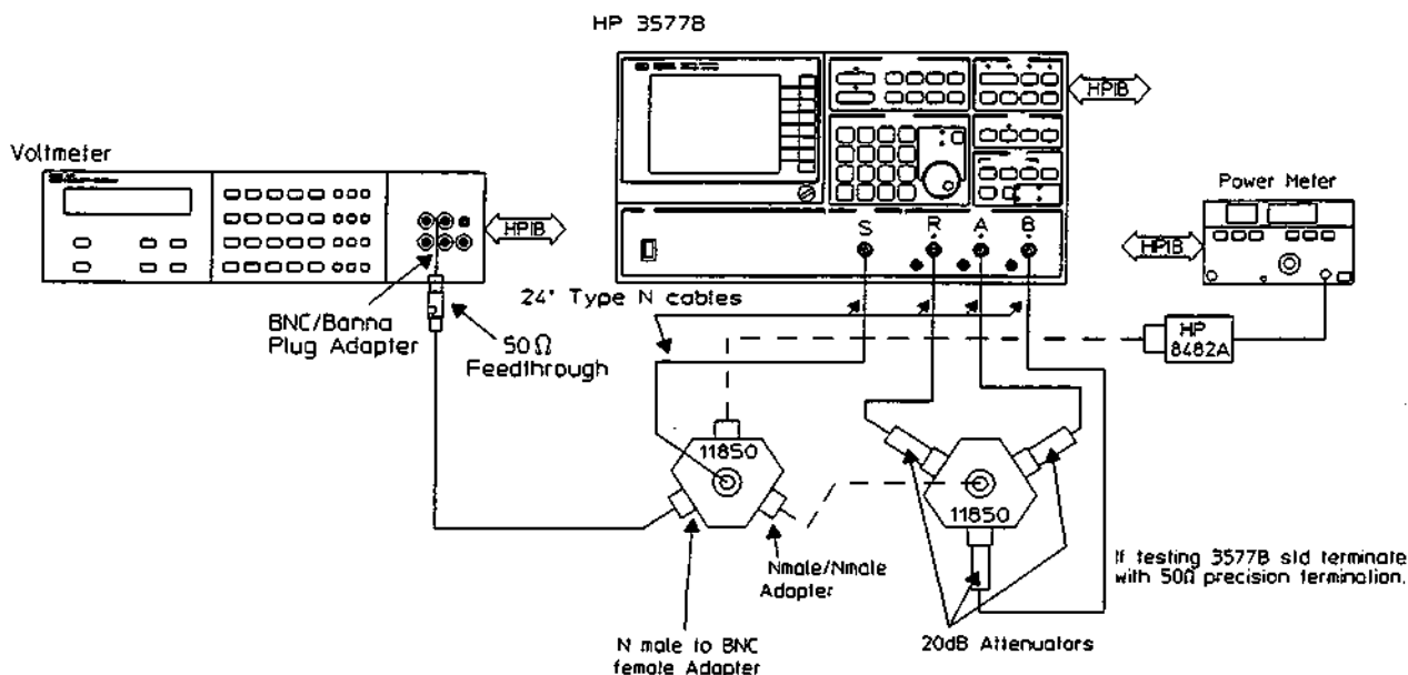
Figure 3-11. Absolute Accuracy and Flatness Test Set-Up (50Ω)
