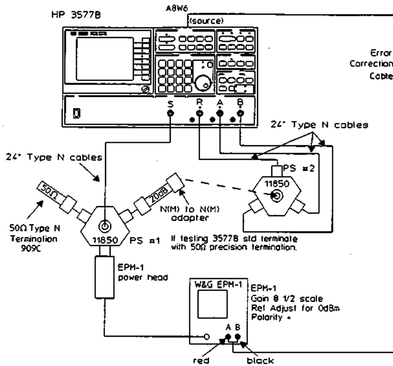
Figure 3-8. Receiver Flatness and Absolute Accuracy Test Set-Up (50 Ω)
