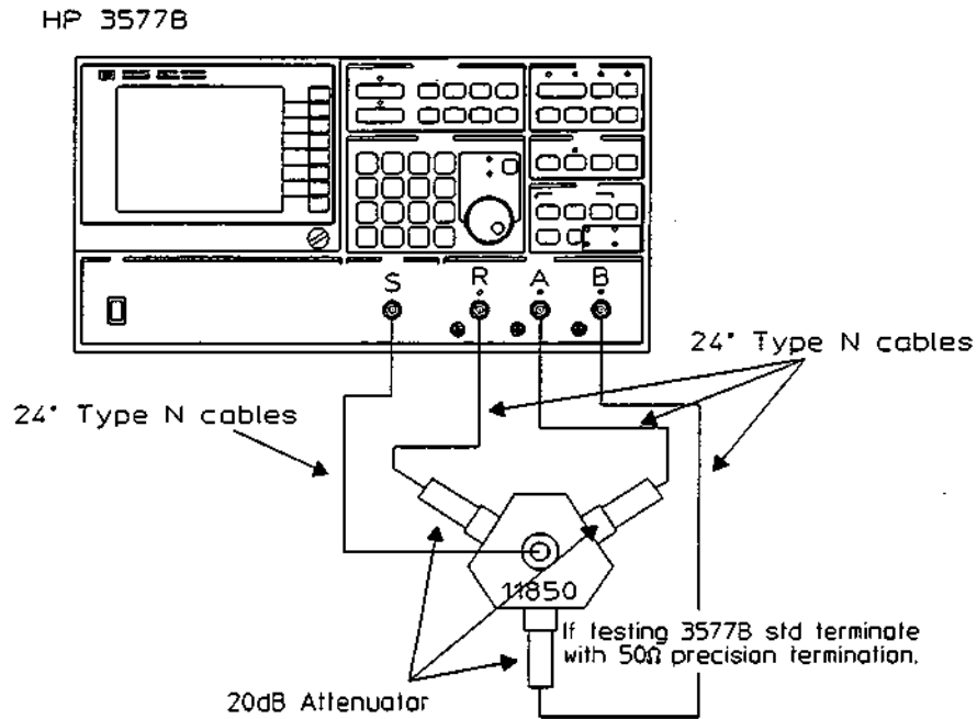
Figure 3-10. Receiver Power Splitter Calibration
