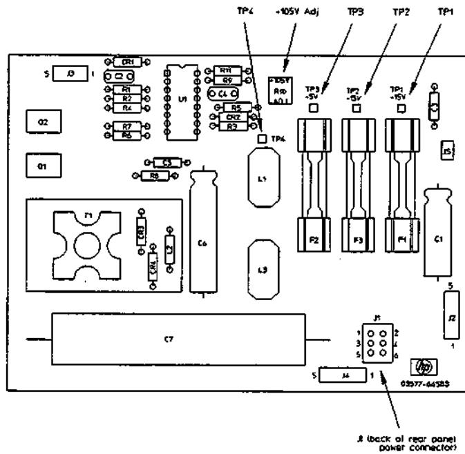
Figure 5-10. A83 Adjustment Locations for Low Voltage Power Supply
