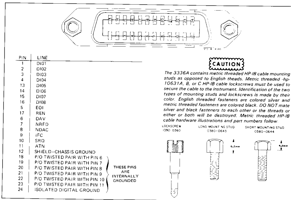
Figure 2-2. HP-IB Connector.
