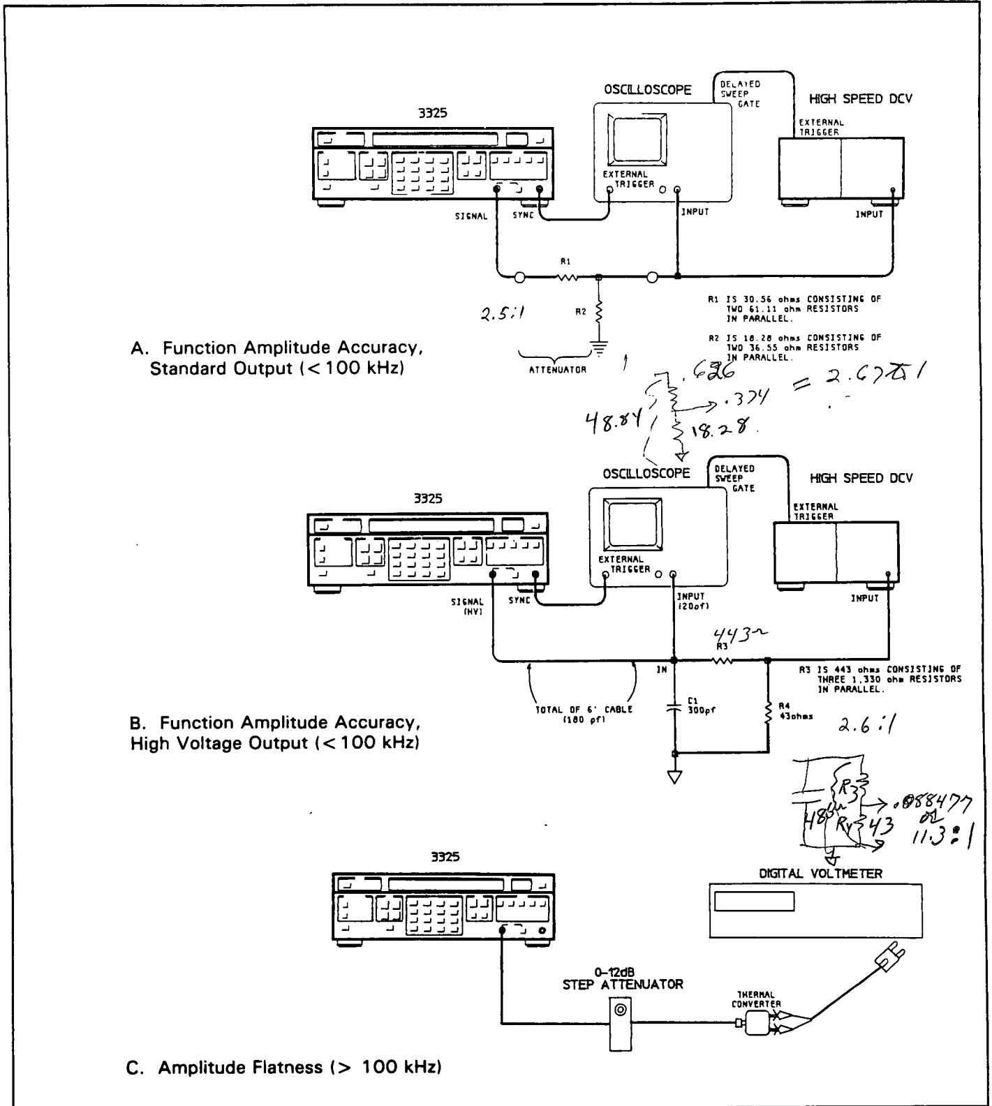
Figure 4-14. Amplitude Accuracy and Flatness.
