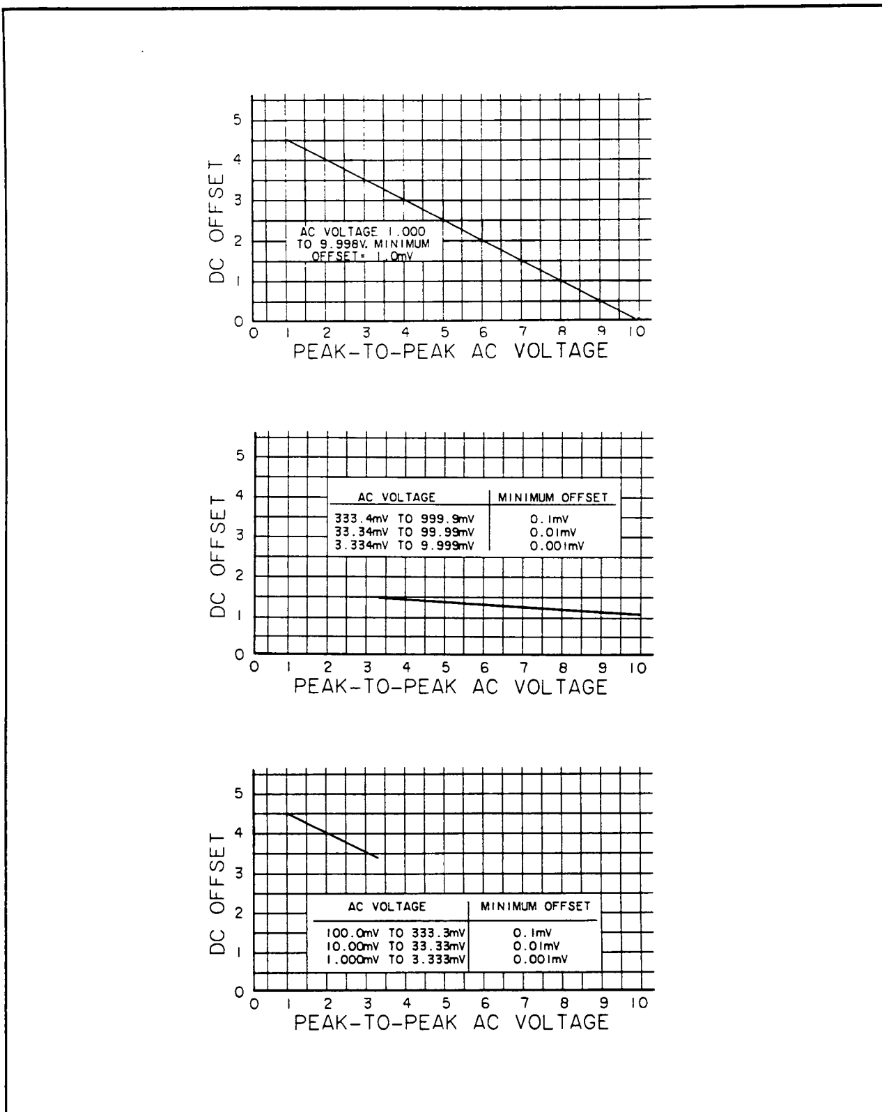
Figure 1-2. Maximum DC Offset with any AC Functions
