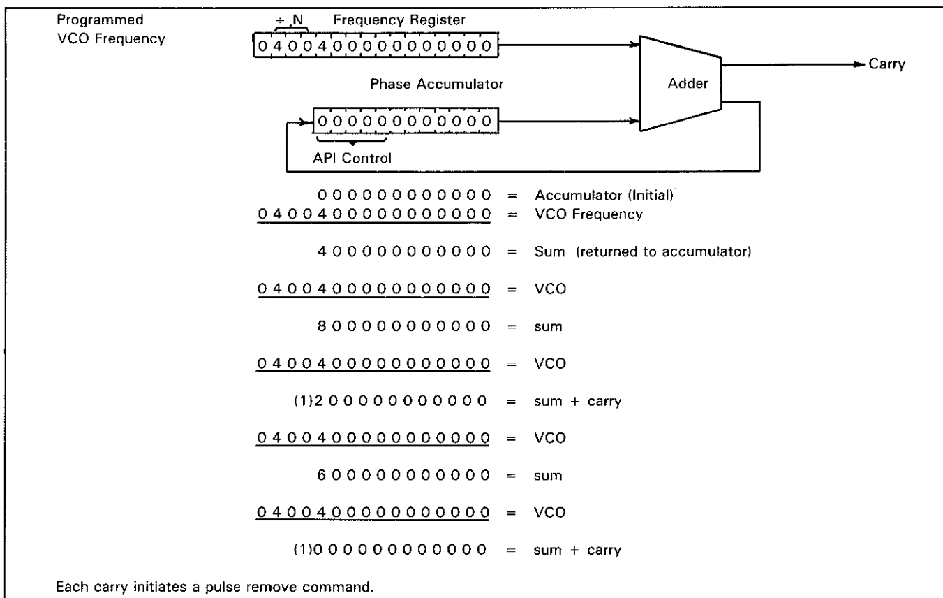
Figure 8-12. Phase Accumulation.
