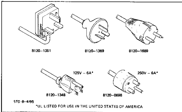
Figure 2-2. Power Cables.
