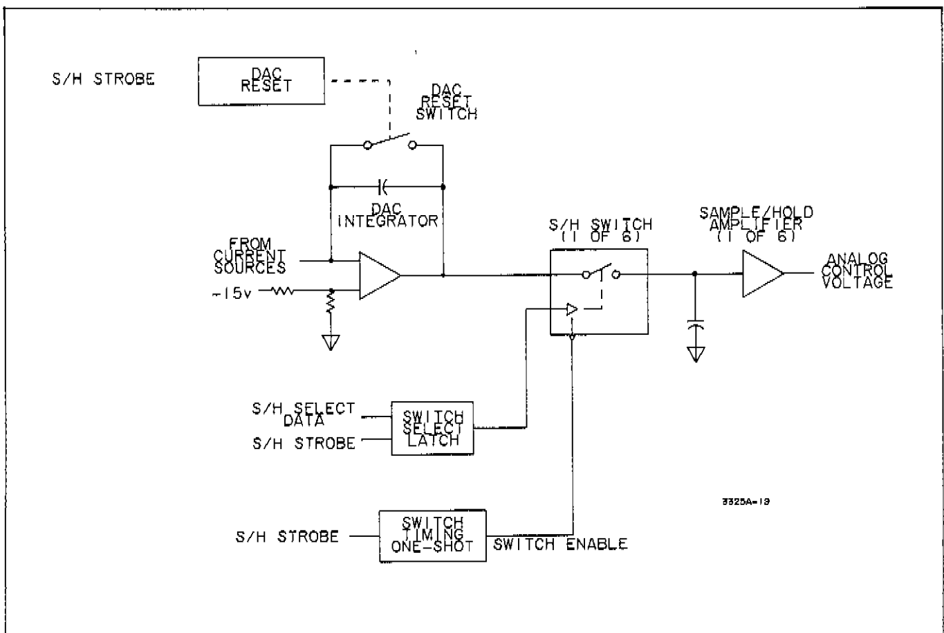
Figure 8-19. DAC Sample/Hold.
