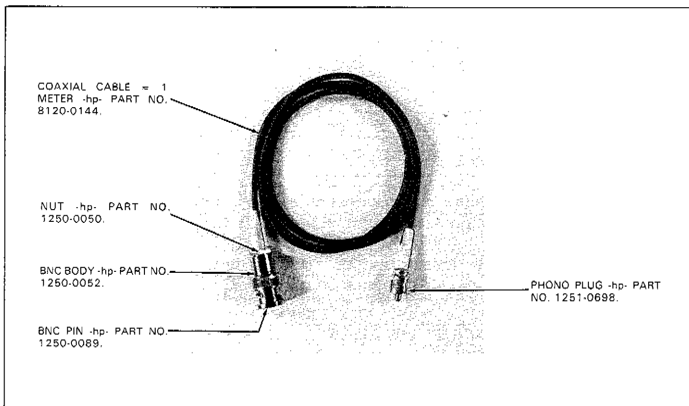
Figure 8-27. Adapter Cable.
