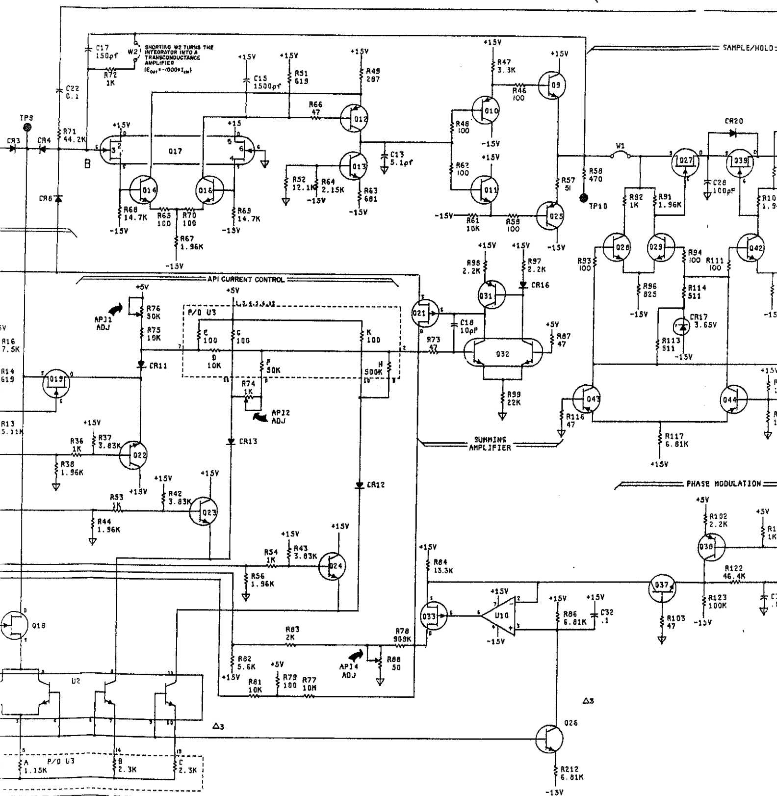
INTEGRATOR
