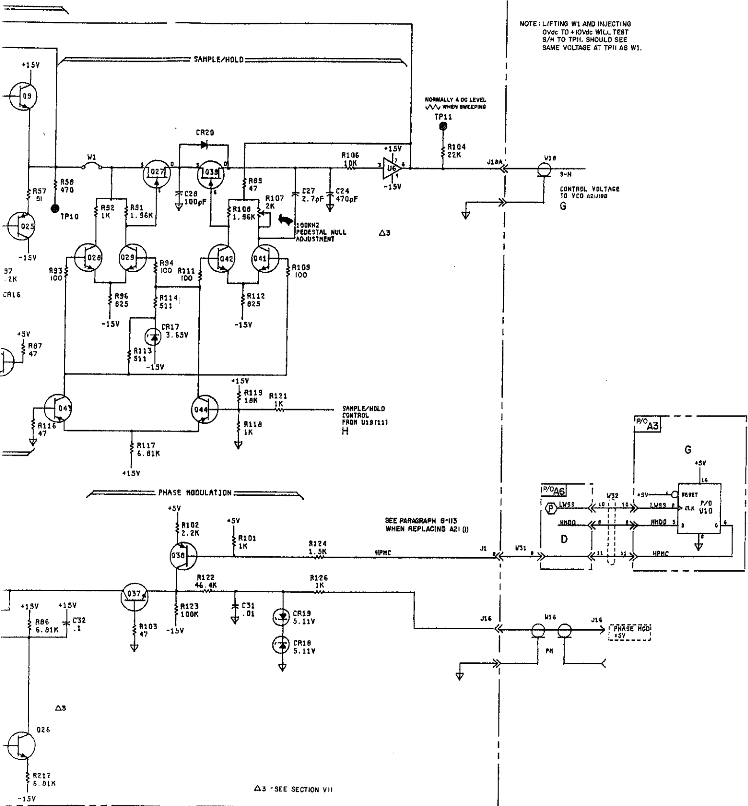
Figure 8-39. Fractional N Analog, A21. 8-F-5/8-F-6
