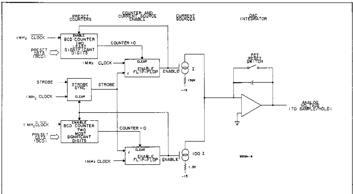
Figure 8-18. D/A Converter.
