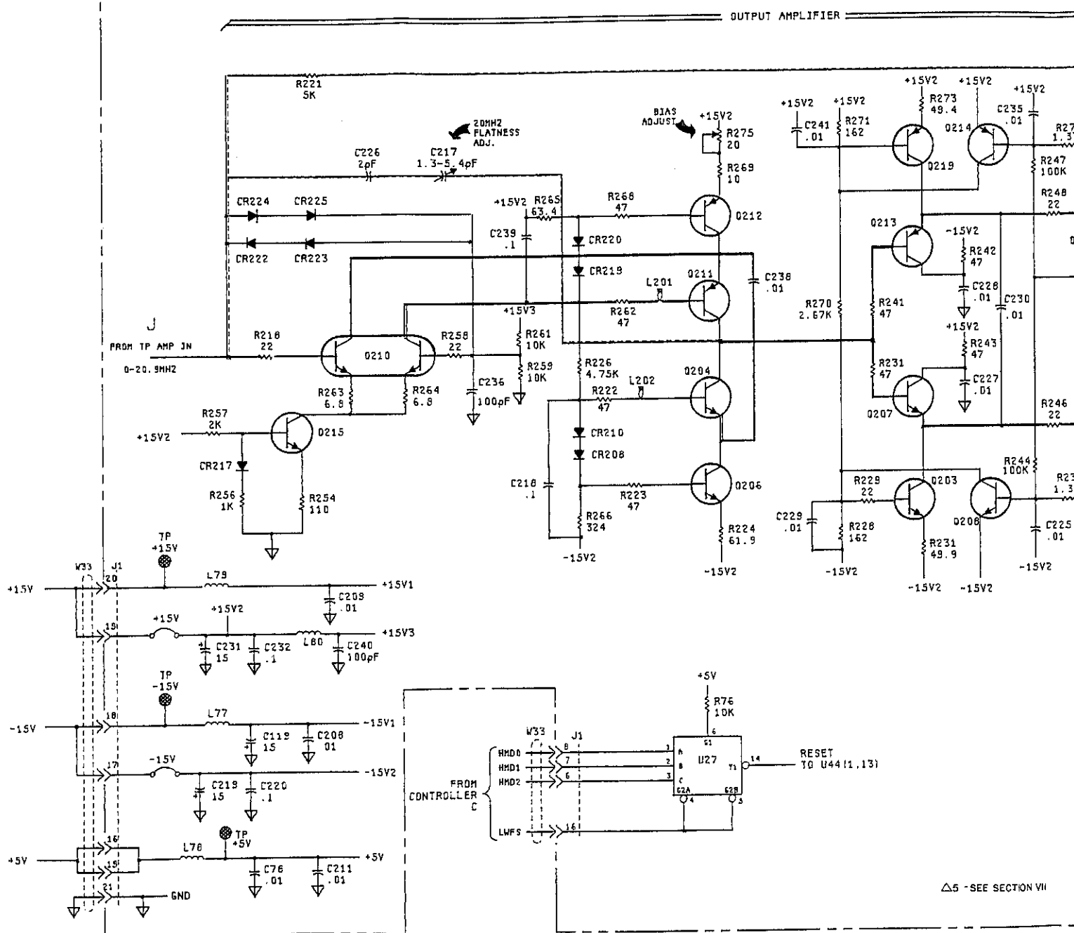
A14 03325-66514 OUTPUT AMPLIFIER
