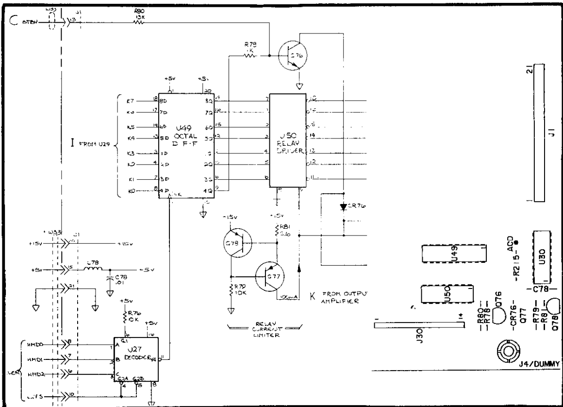
Figure 7-18. Relay Drive Circuitry (Serial Numbers 1748A01075 and Below).
