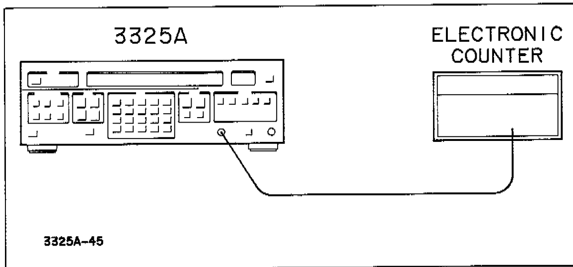
Figure 4-6. Frequency Accuracy.
