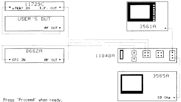
Figure 6-11. HP 11729C/HP 8662A with EFC Tune Voltage
