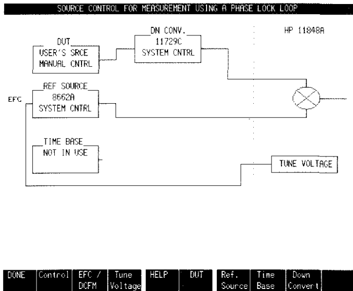
Figure 6-17. EFC Tune Voltage Tuning with HP 8662A 640 MHz Reference
