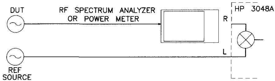
Figure 2-12. R Port Power Setup Diagram
