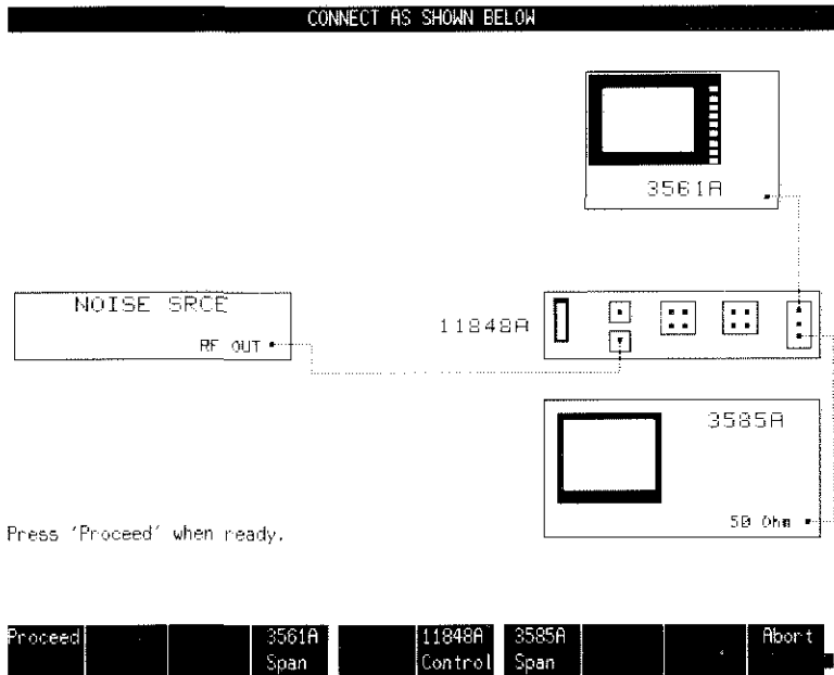
Figure 2-6. Block Diagram of the Baseband Noise Measurement
