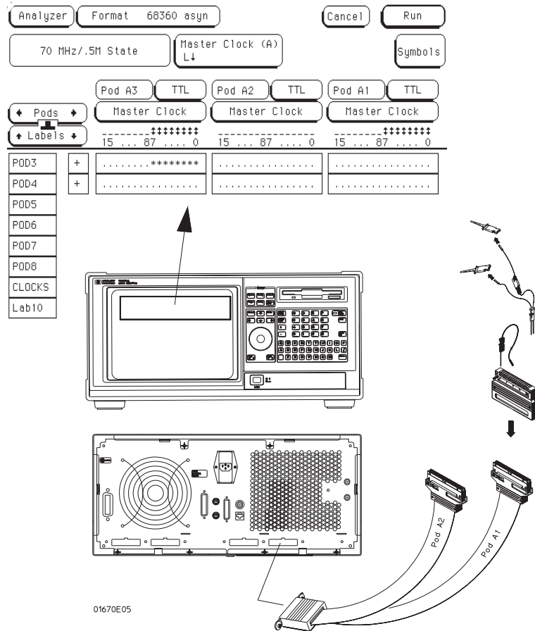
Connecting ProbeCables to the LogicAnalyzer
