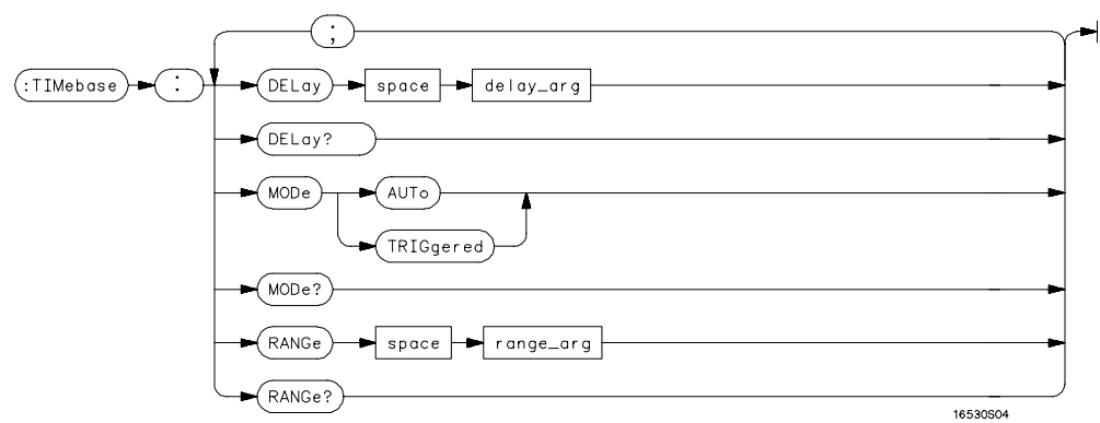
TIMEbase Subsystem Syntax Diagram
