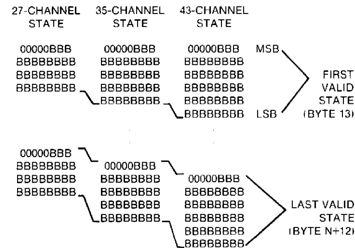
Figure C-1. Data Format For State Acquisition Learn String Sent On HP-IB
