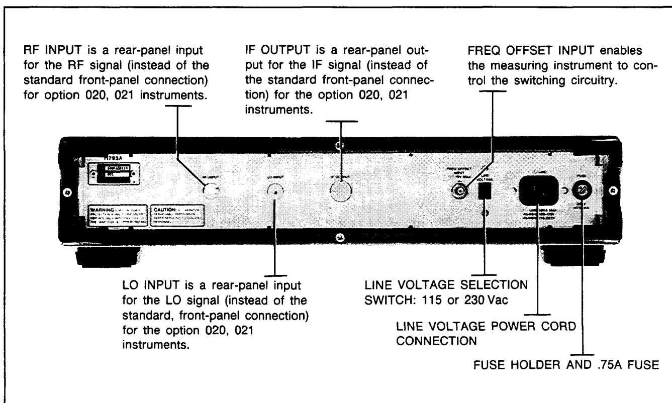
Figure 5. Rear-Panel Features
