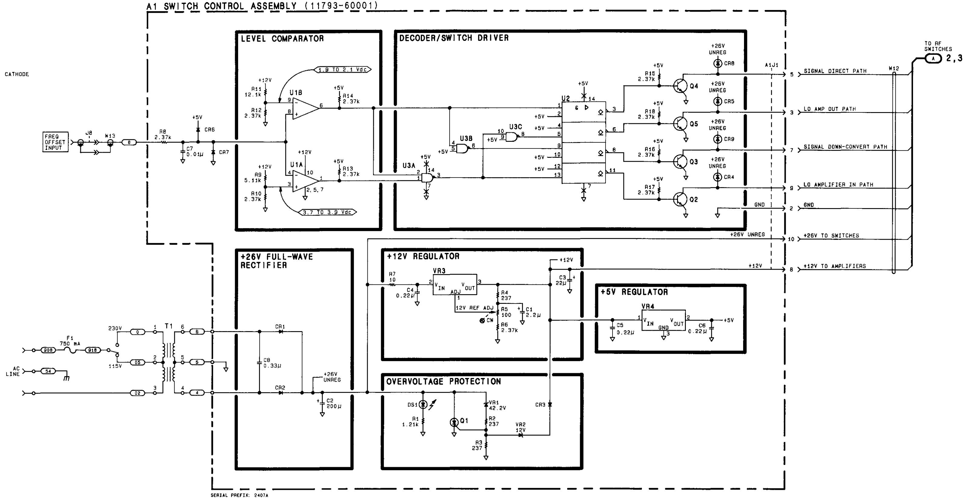
SS3 Figure 14. A1 SWITCH CONTROL ASSEMBLY, Schematic Diagram 43/44
