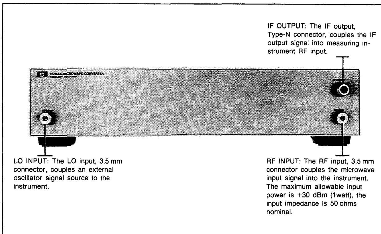
Figure 4. Front-Panel Features
