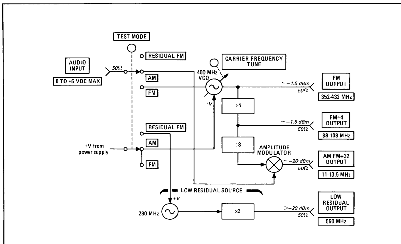
Figure 1-2. HP Model 11715A Test Source Block Diagram
