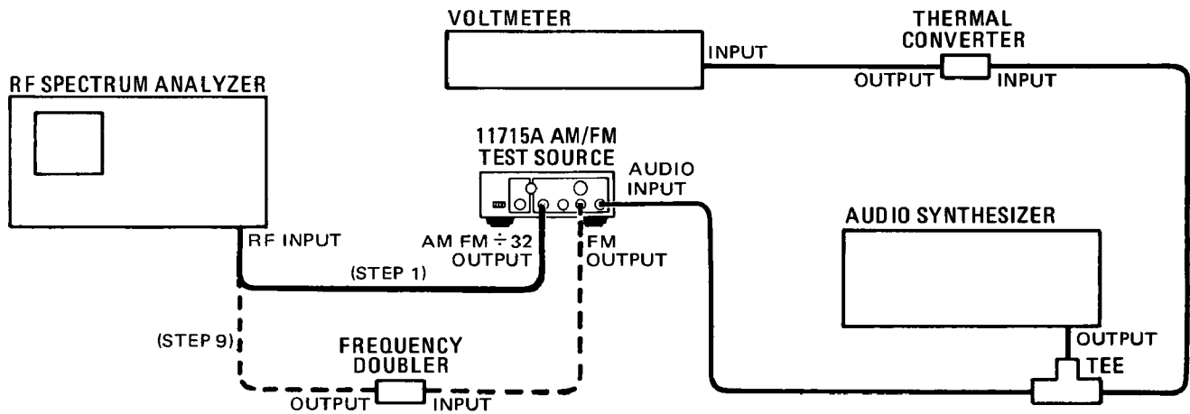
Figure 4-3. FM Flatness Test Setup
