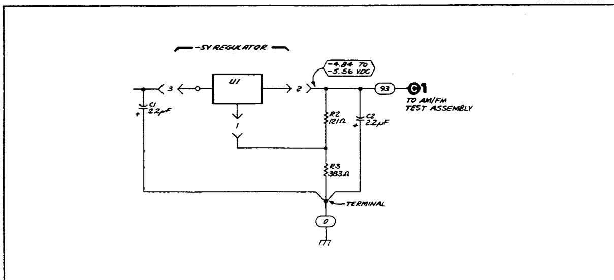
P/O Service Sheet 2 (Schematic). -5 Volt Regulator Circuit (P/O Change 1).
