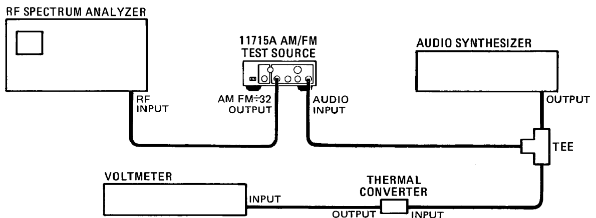
Figure 4-7. High-Frequency AM Flatness Test Setup
