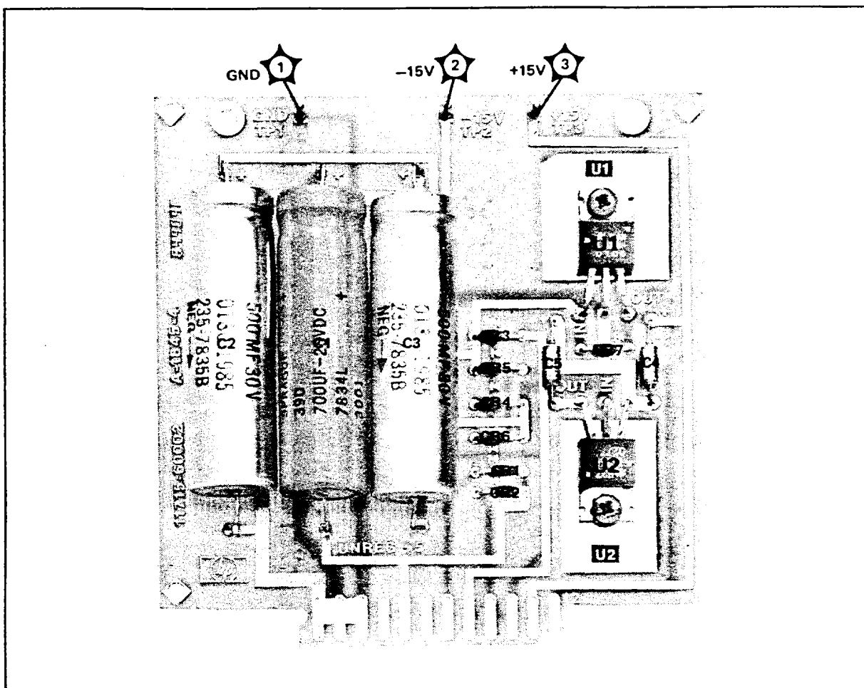
Figure 8-5. A2 Power Supply Assembly Component Locator (P/O Errata)
