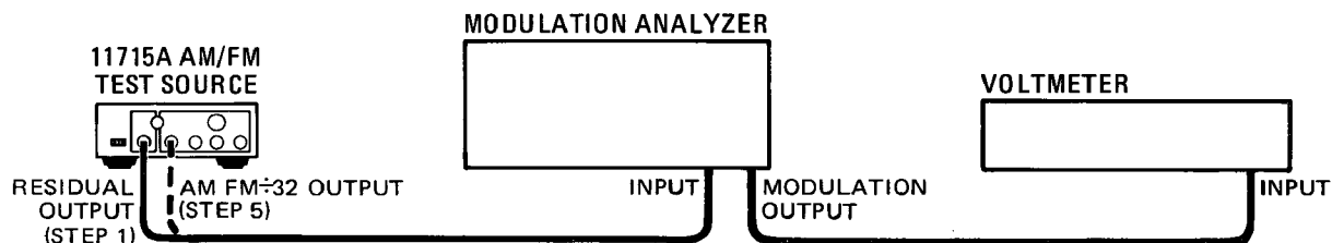
Figure 4-1. Residual FM and AM Test Setup
