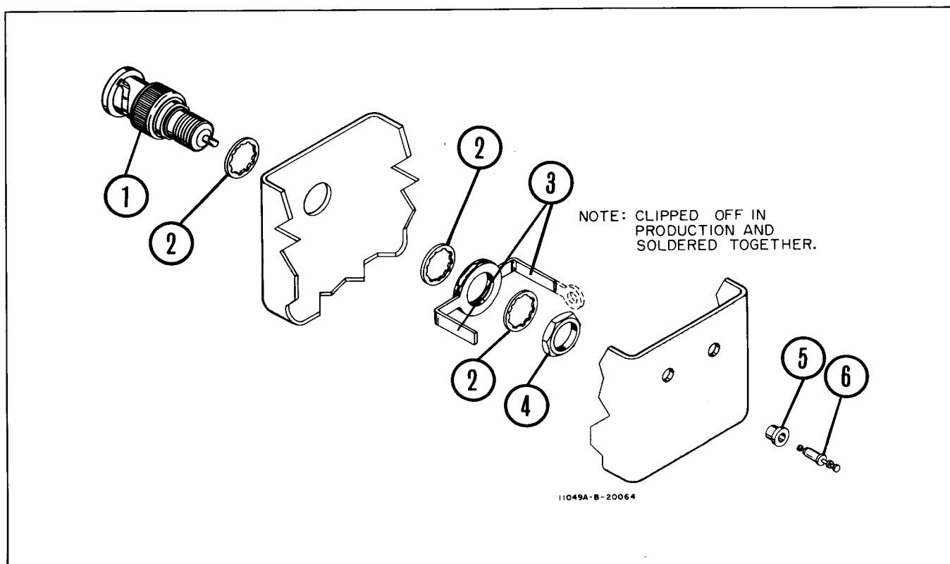
Figure 9. Mechanical Parts
