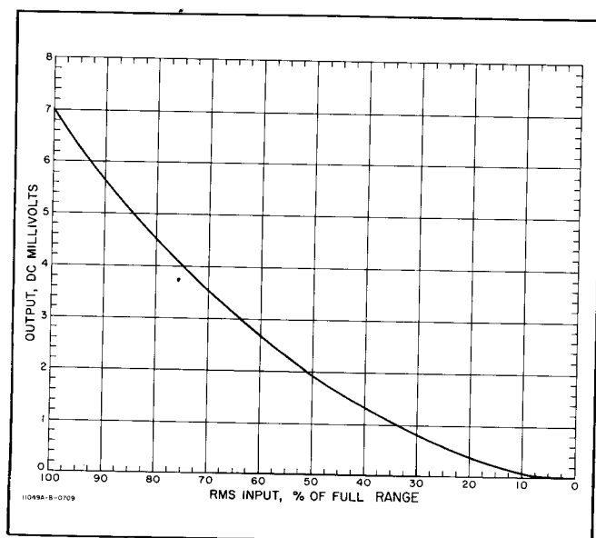
Figure 3. Input/Output Relationship
