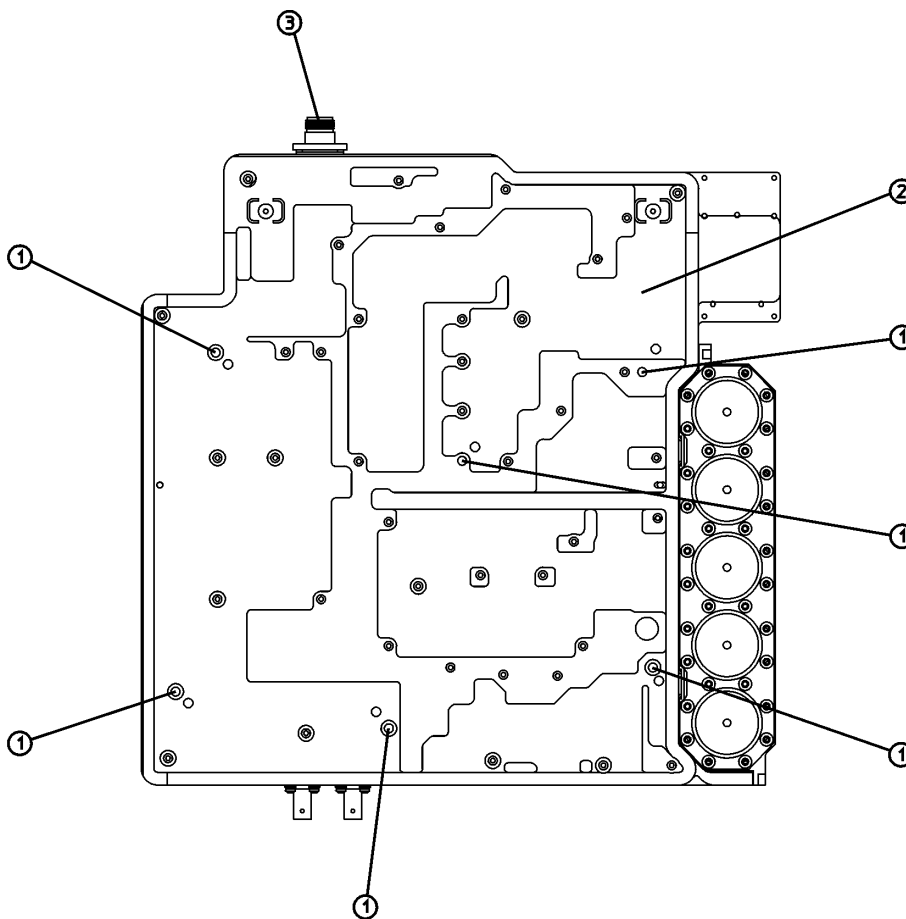
RF Assembly with Hardware, E4401B and E4411B
