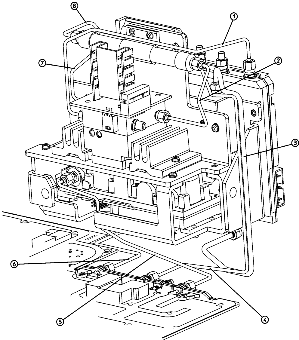
Microwave RF Assembly Rear View, Semi-rigid Cables E4404B, E4405B, E4407B and E4408B
