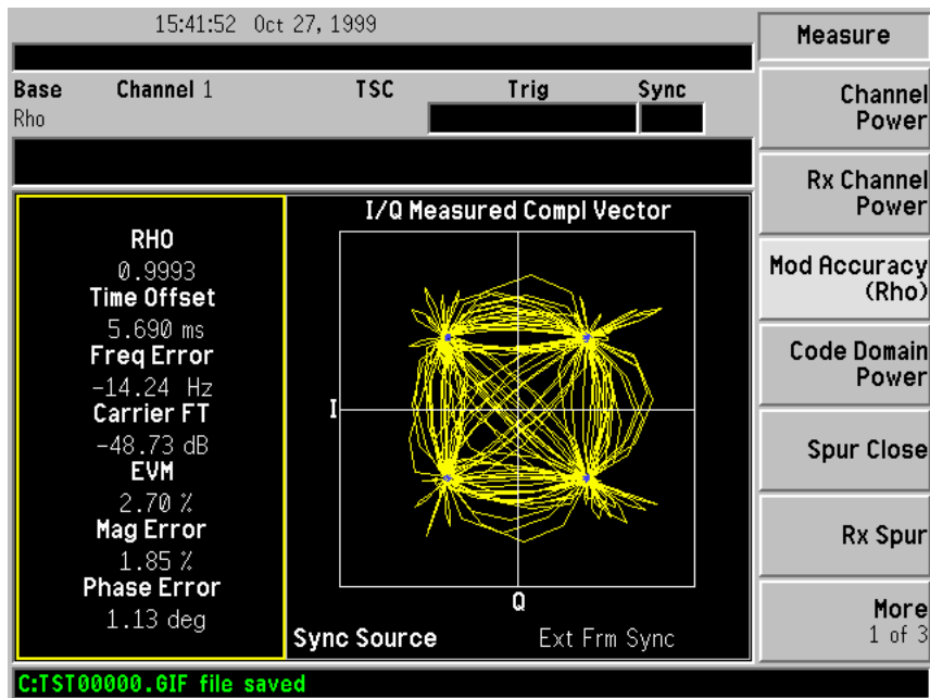
Figure 1-6 Modulation Accuracy (Rho) Display
