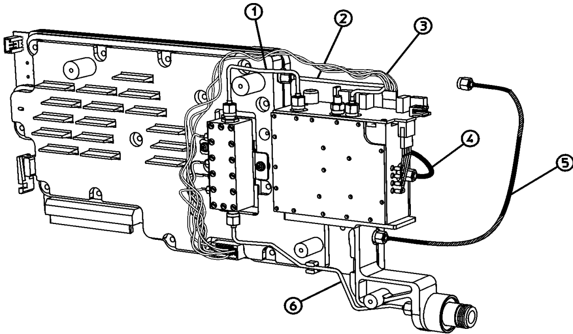
Figure 5-29 3.0 GHz Tracking Generator Assembly with Cables
