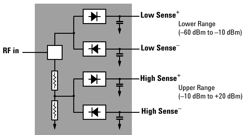
Figure 1-2 Simplified Block Diagram of Diode Pair/Attenuator/Diode Pair
