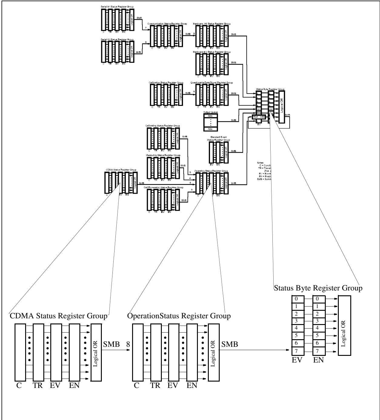
Figure 33 Test Set Data Structures
