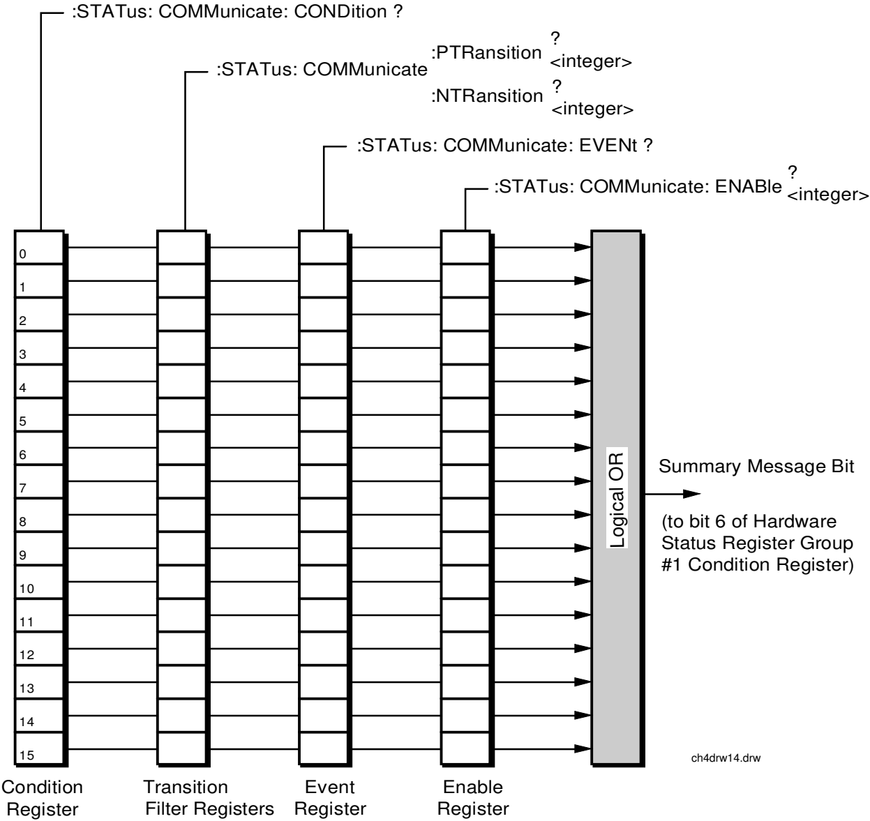
Figure 19 Communicate Status Register Group
