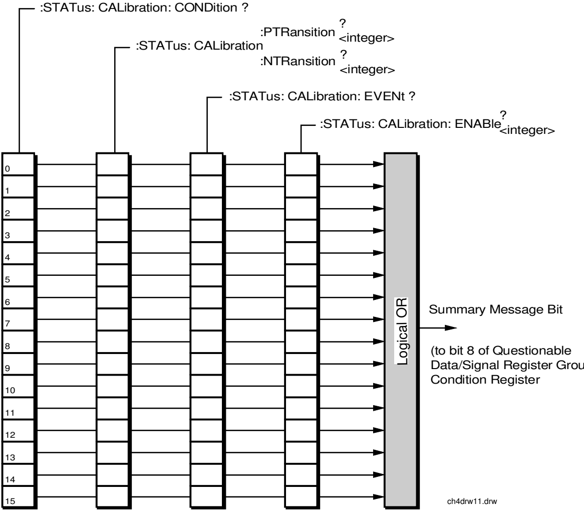
Figure 12 Calibration Status Register Group
