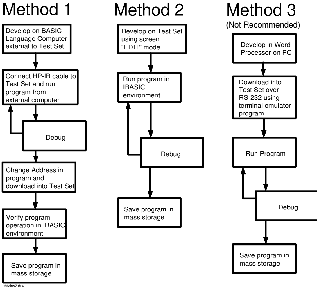
Figure 39 Program Development Methods
