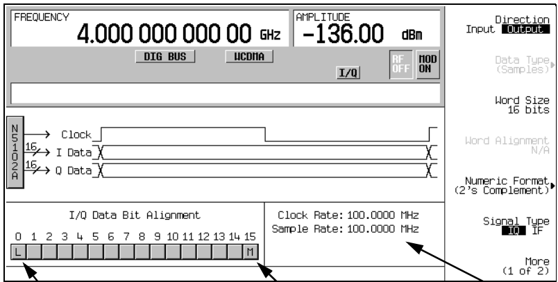
Figure 11-1 Data Setup Menu for a Parallel Port Configuration
