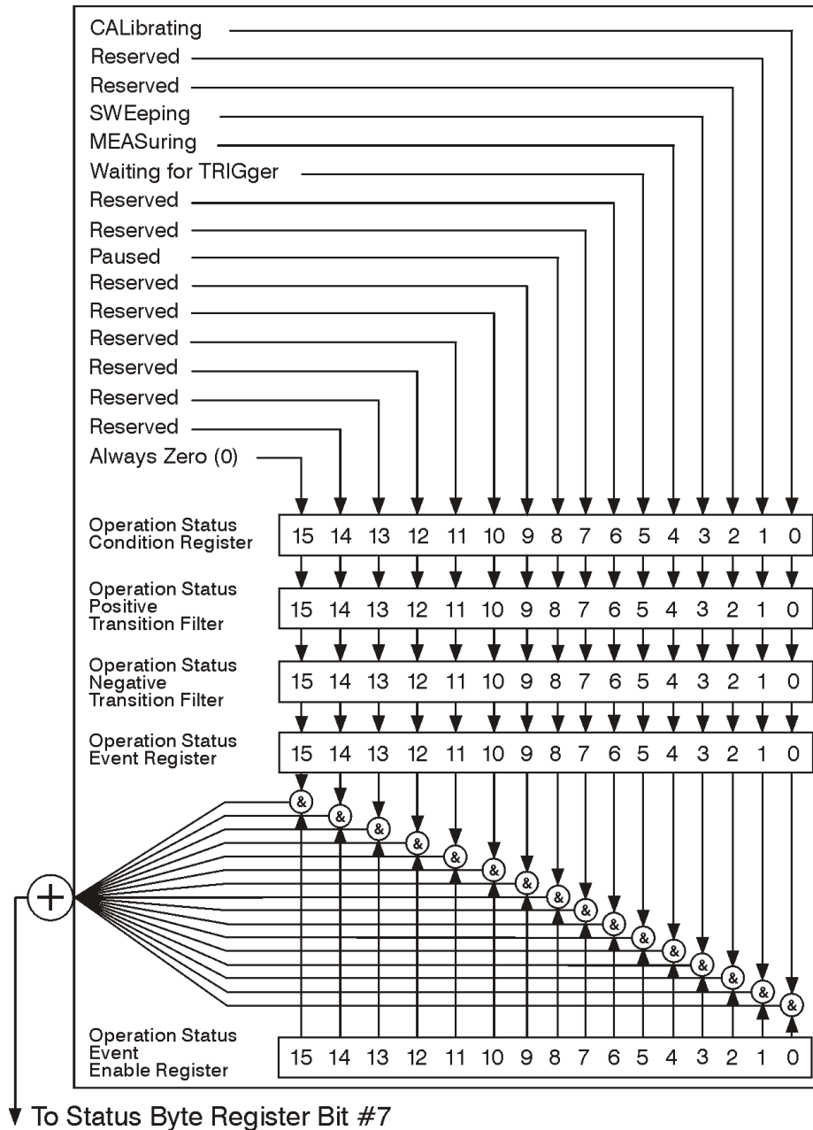
Figure 2-8 Status Operation Register Diagram
