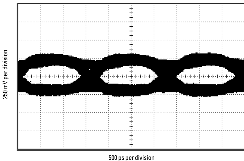
Logic analyzer eye opening for a PRBS signal of 250 mV, 600 Mb/s data rate, 1 ns rise time
