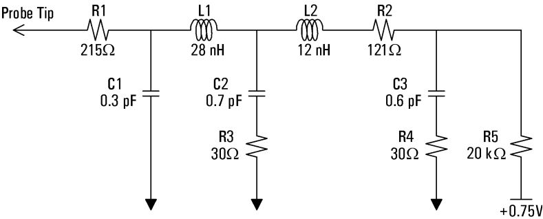
Equivalent load model
