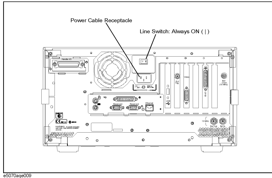
Line switch (Always ON) and power cable receptacle
