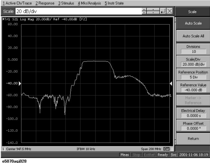
S21 trace after executing the auto scale
