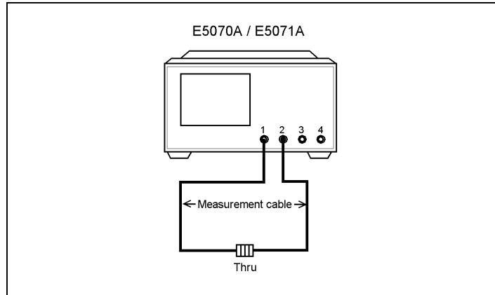
Connecting the THRU standard
