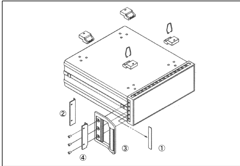
Figure 1-4 Mounting the handle/rackmount kit
