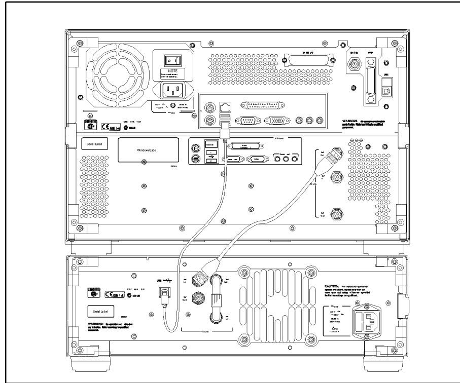
Figure 3-2 Connecting E5052A and E5053A (Rear Panel)
