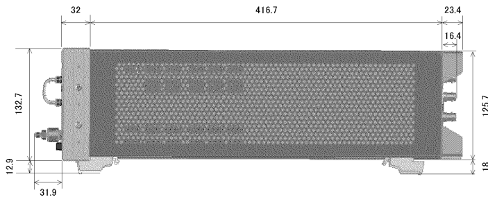
Figure 10-8. Side view
