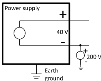
Example of negative terminal floating +200 V above ground (positive terminal is +240 V above ground)
