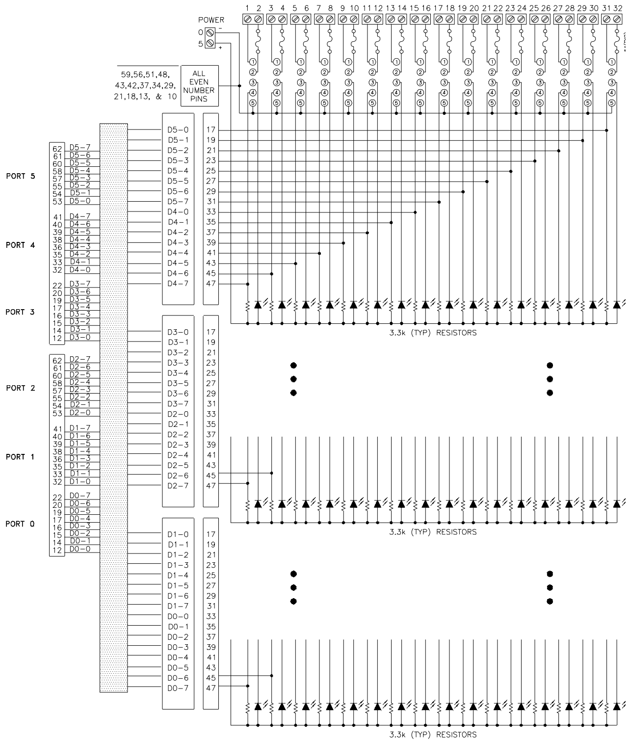
Figure 2-8. Opto 22 Connections
