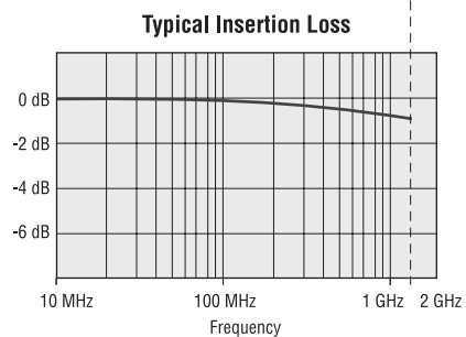
75 \Omega Mux Typical AC Performance Graphs
