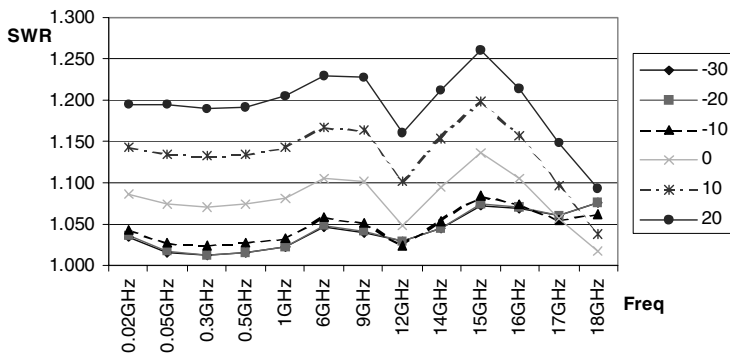
Figure 4 Typical SWR (50 MHz to 18 GHz) for the E9323A and E9327A sensors at various power levels
