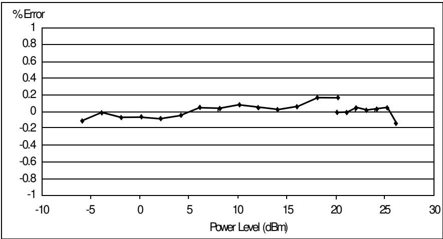
Figure 17 E9300B Typical Power Linearity at 25°C, after zero and calibration with associated Measurement Uncertainty
