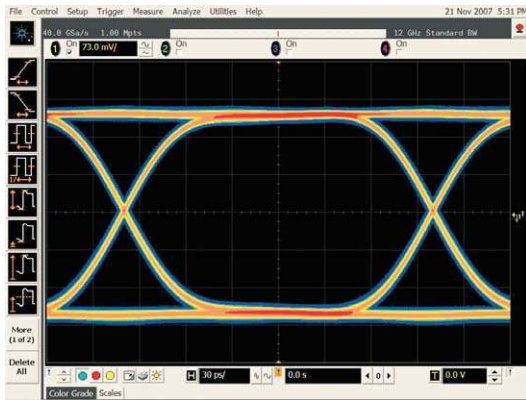
5 Gbps PCI EXPRESS Gen 2 eye pattern. The ultra-low noise floor of DSA91204A shows the true performance of your device under test.
