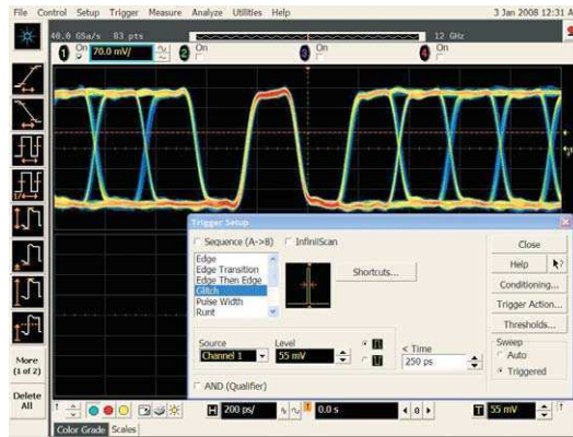
Consistently trigger on 200 ps single bit (one UI) of PCI EXPRESS Gen 2 using industry-leading < 250 ps glitch trigger.
