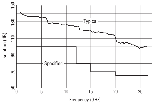
Figure 8. Isolation
