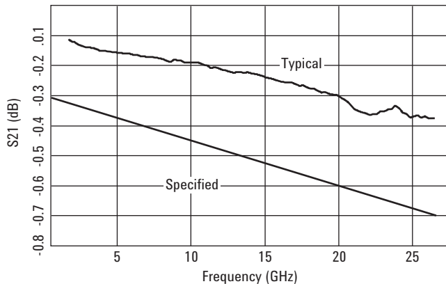
Figure 7. Insertion loss
