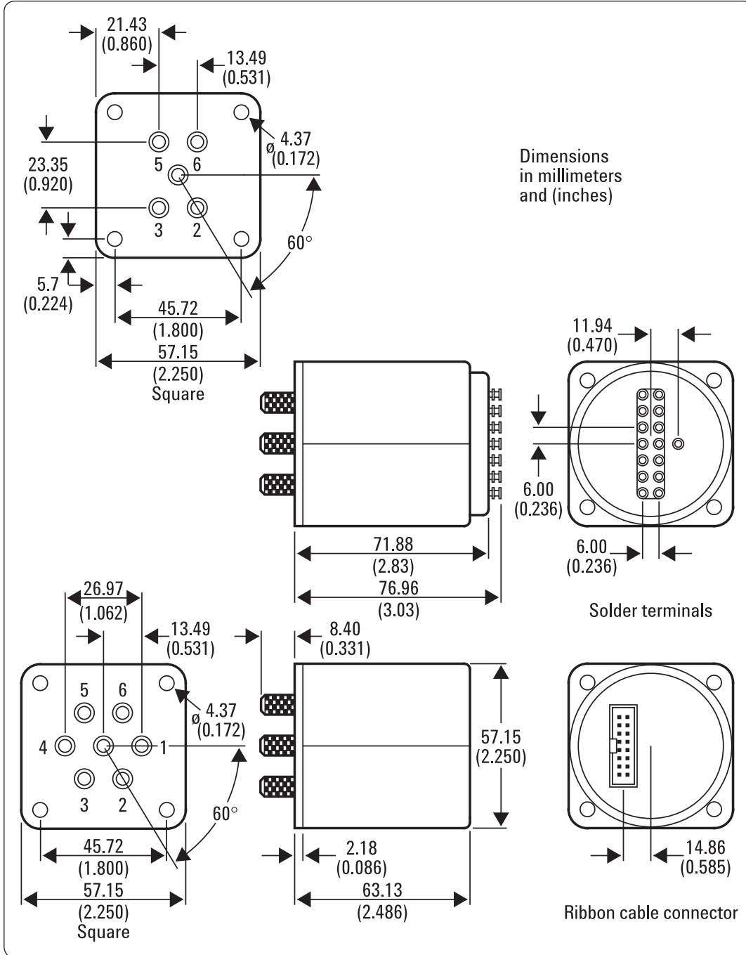
Figure 9. Product outlines
